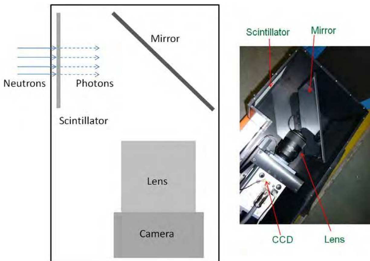
Fig. 6. Scintillator based neutron imaging device.
