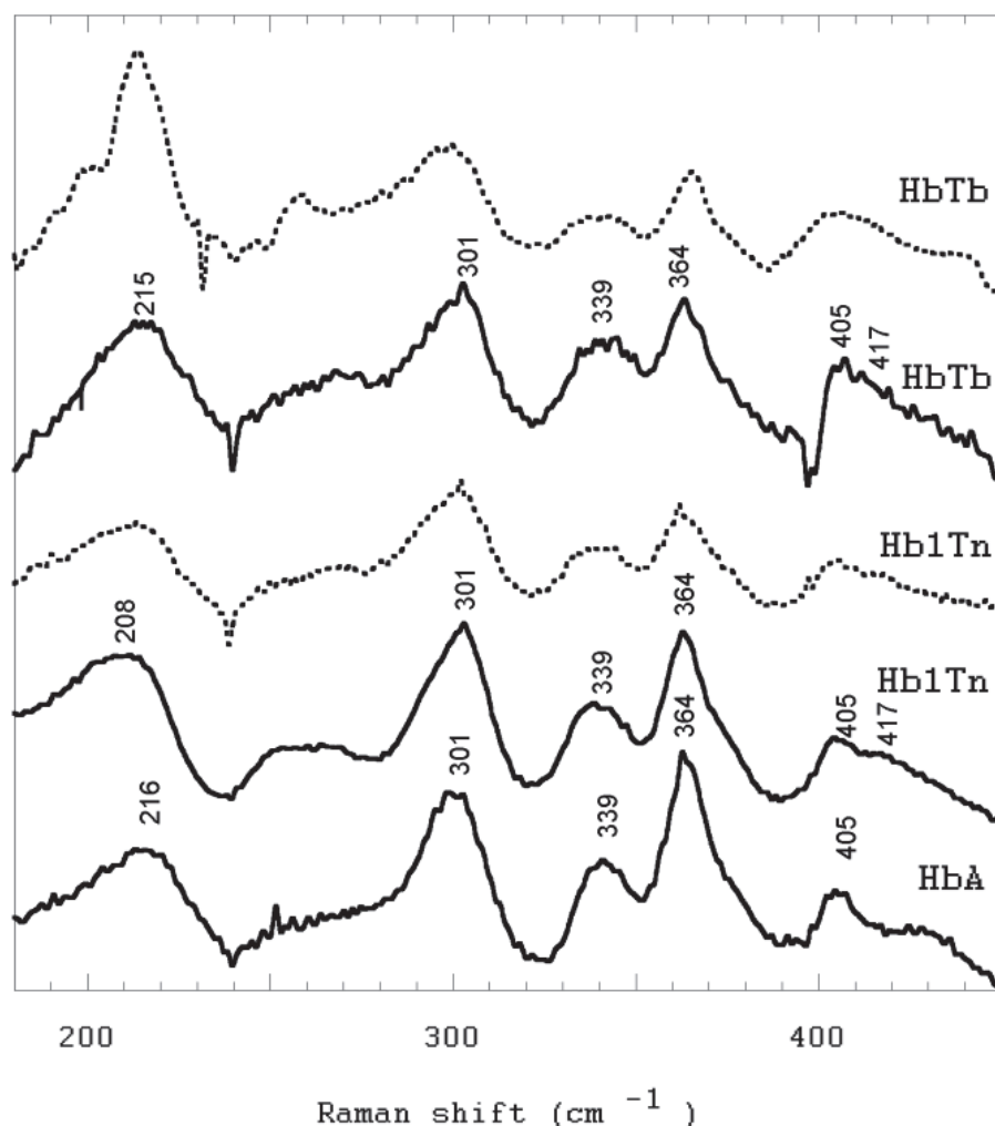
Fig. 5. Resonance Raman spectra in the low-wavenumber region of Hb1Tn (major hemoglobin of T. newnesi ) both in solution (solid lines) and in the crystal state (dashed lines) in the deoxy state. As reference of usual coordination also HbTb (major hemoglobin of T. bernacchii ) and human HbA are reported (After Vergara et al., 2010).
