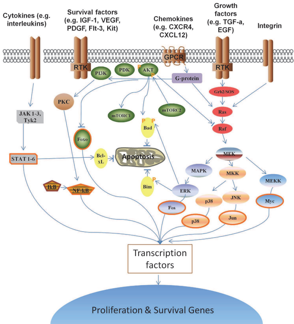
Fig. 1. Signal transduction pathways (refer text for details)
