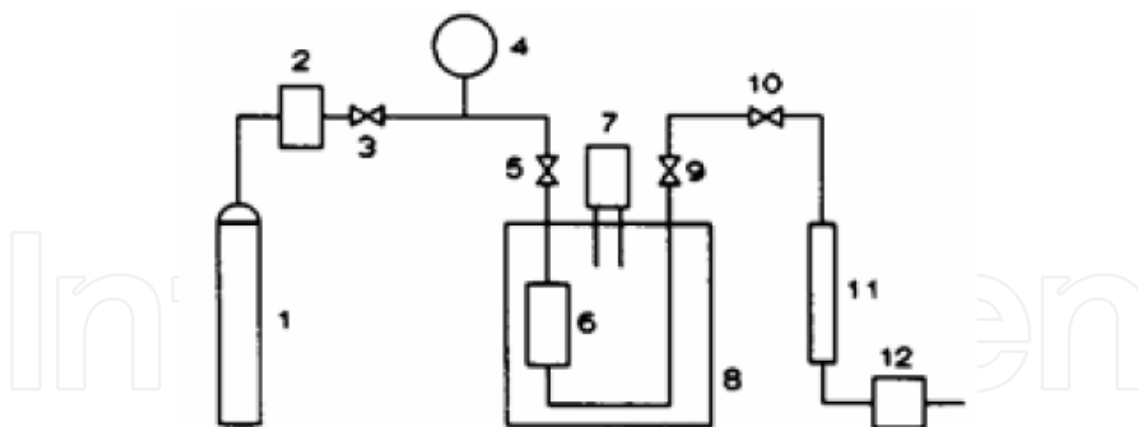
Fig. 8. The supercritical carbon dioxide apparatus used for dyeing of synthetic fibers 1. Liquid CO 2 , 2. Pump, 3,5,9. Pressure-control valves, 4. Manometer, 6. Autoclave, 7. Temperature sensor, 8. Dyepot, 10. Adjust valve (Li-qiu et al., 2005)
