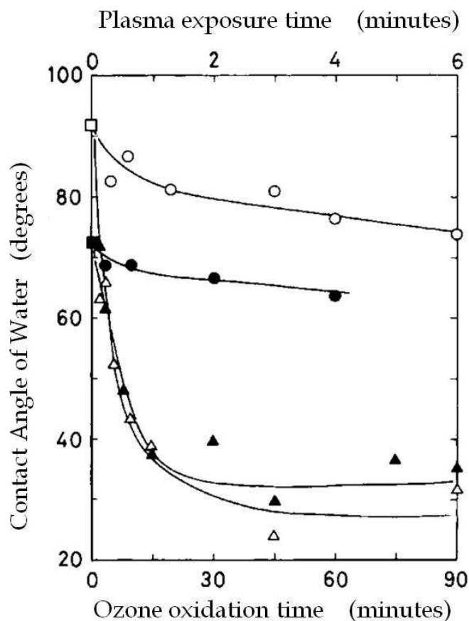
Fig. 6. Decrease in contact angle of PE and PU films by ozone oxidation and plasma exposure. Ozone (60V, 50 Lhr -1 ): (○) PE, (●) PU. Plasma (Ar, 24 W): (△) PE, (▲) PU. Virgin: (□) PE, (■) PU. From (Fujimoto et al., 1993).
