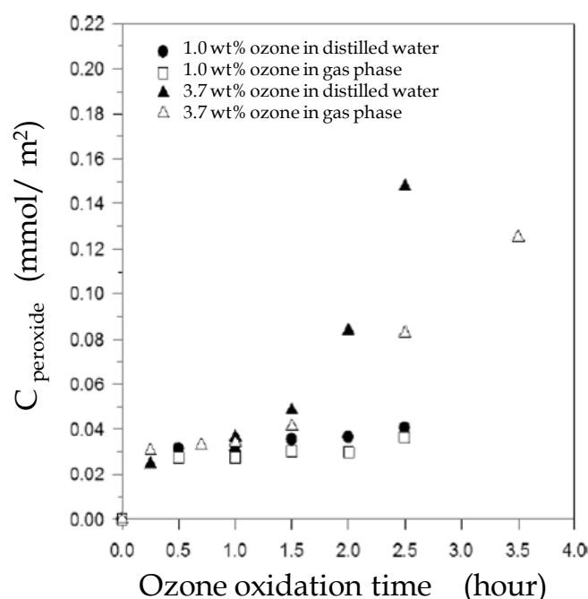
Fig. 7. Peroxides generated after different ozonation times in different media (Gu et al., 2009)
