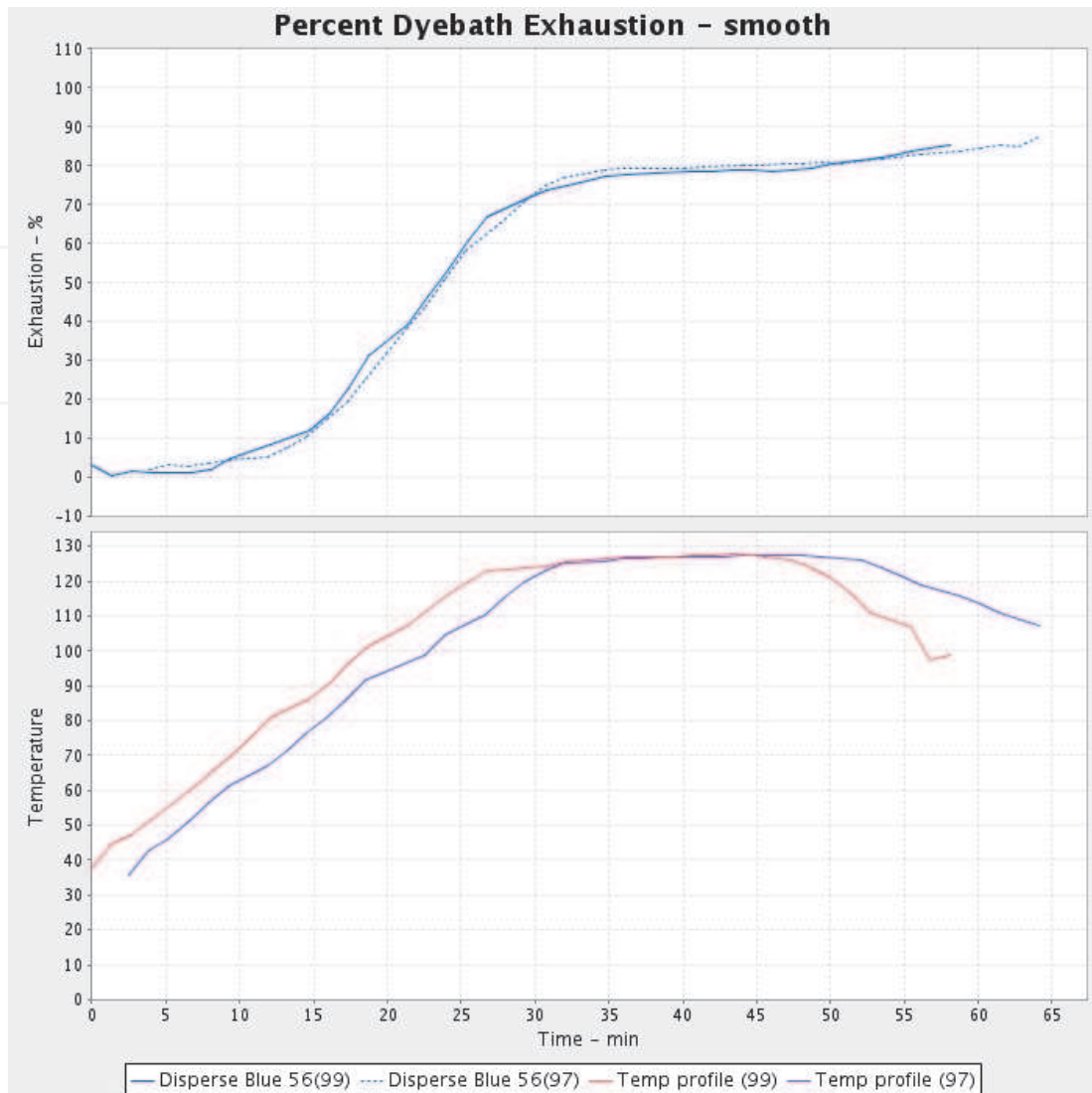
Fig. 9. Different yarn used in same fabric structures.
