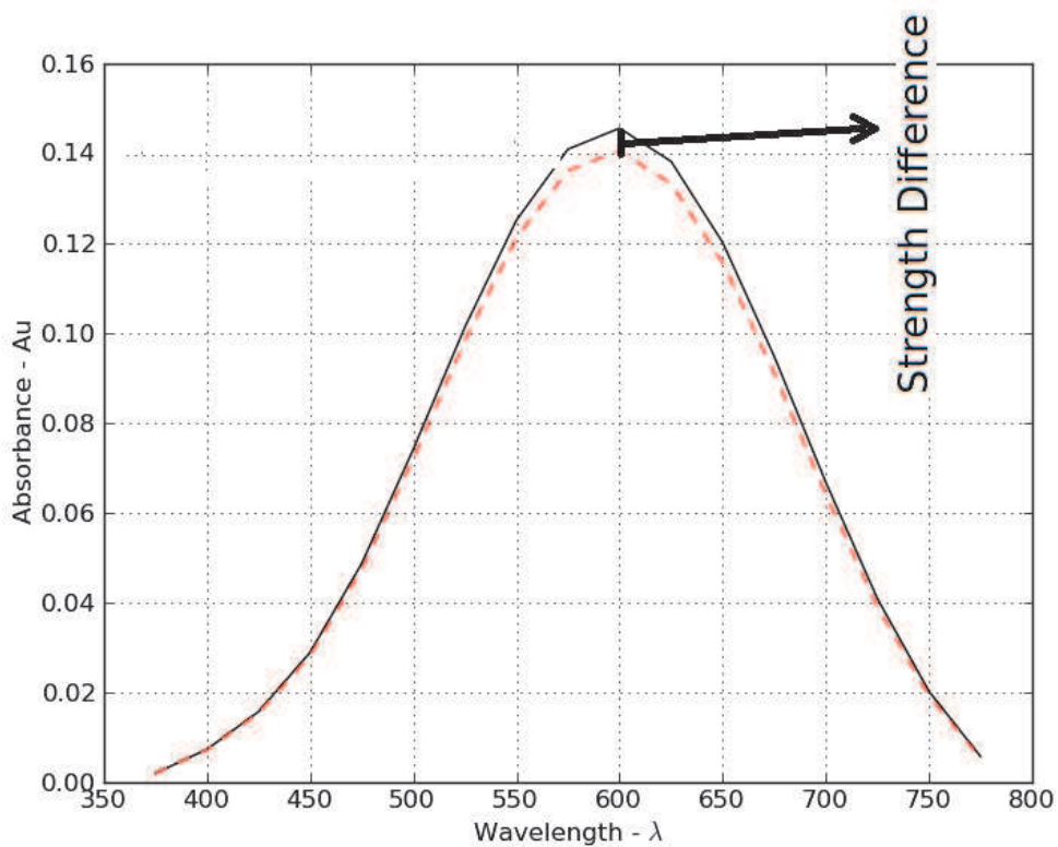
Fig. 5. Strength differences in dyes.
