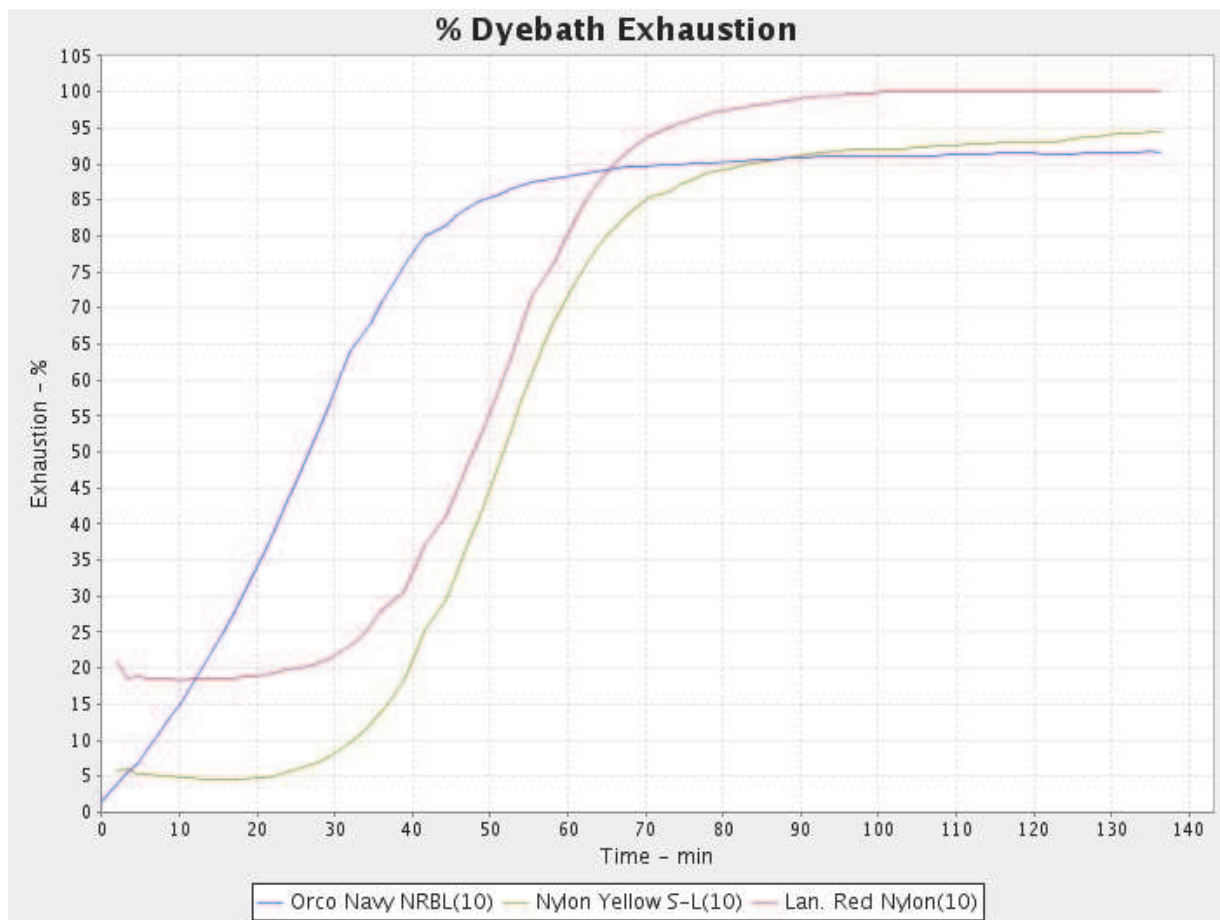
Fig. 15. Incompatibilities between dyes.
