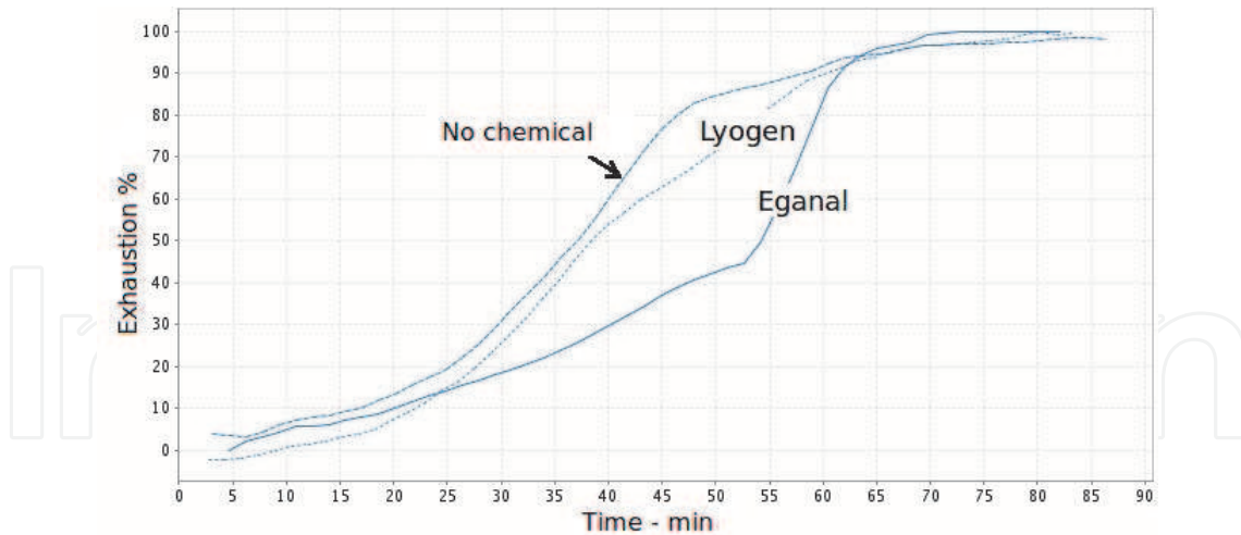
Fig. 11. Effect of leveling agent on dyeing
