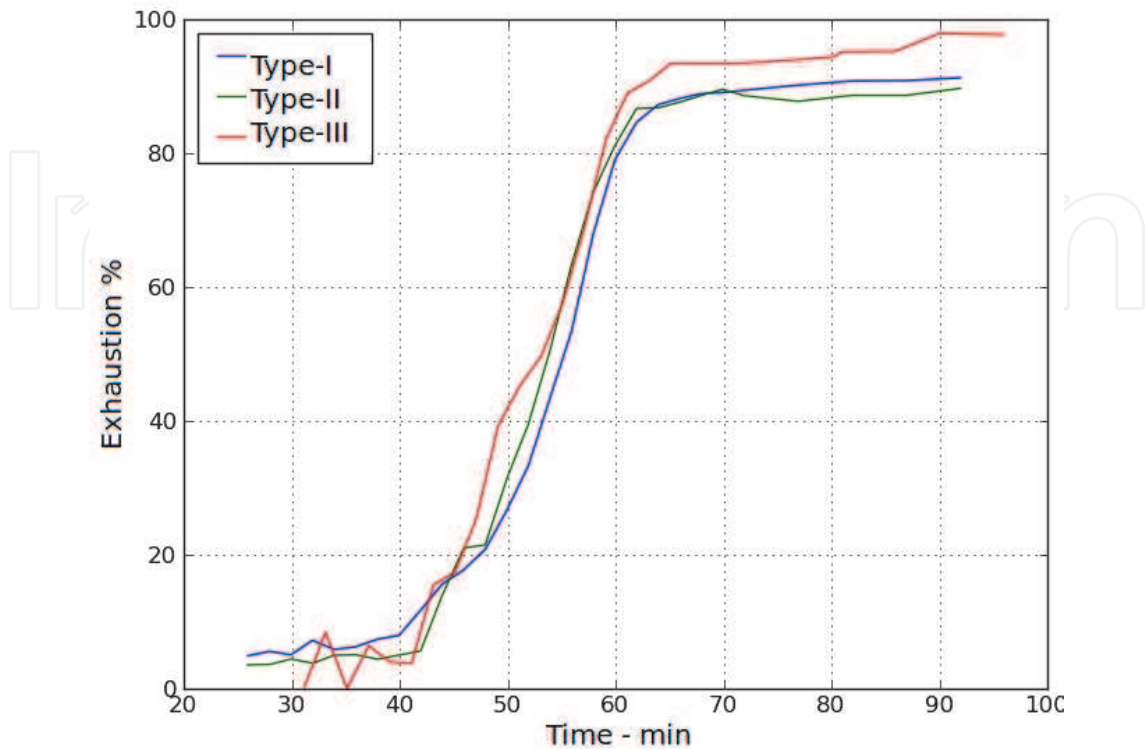
Fig. 7. The exhaustion curves of three shipments of the polyester fiber.
