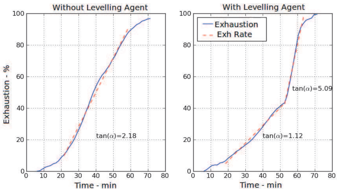
Fig. 12. Effect of leveling agent on dye strike rate
