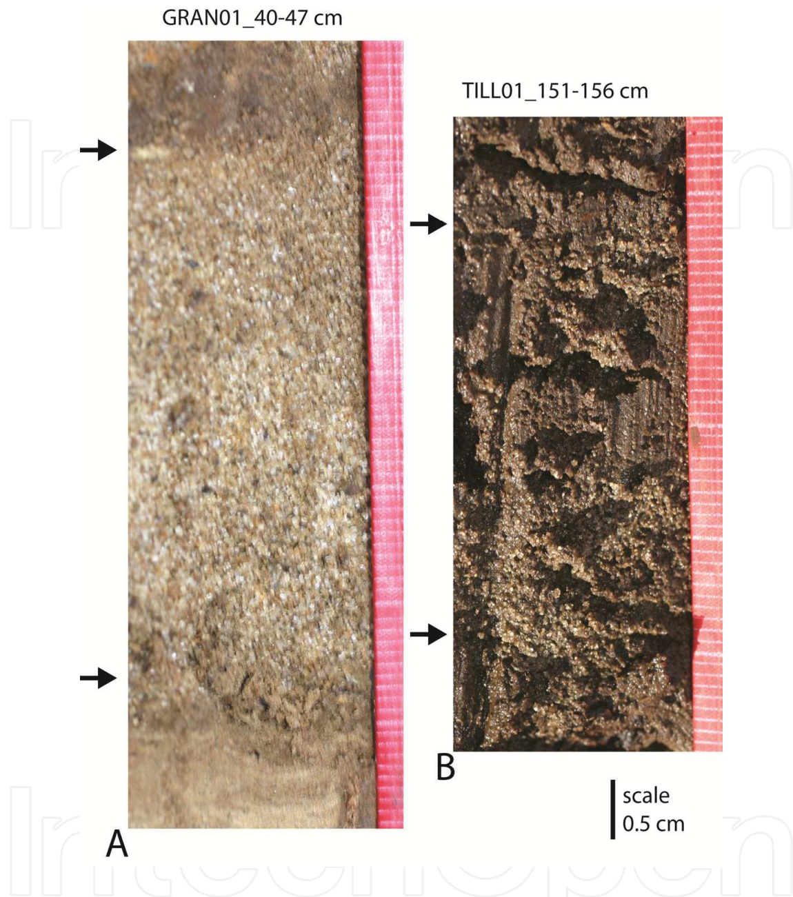
Fig. 3. Contrasting paleotsunami sand layers shown between black arrows for (A) Grant Creek (40-47 cm depth at core site GRAN1) and (B) Tillicum Creek (151-156 cm depth at core site TILL1). The sand sheet deposit from Grant Creek (5-6 cm thick) shows 1) an undisturbed tsunami sand layer (TSL), 2) clear contrast with oxidized hosting alluvium, 3) a sharp bottom contact, 4) fining-upward grain-size trend, and 5) a dark organic-rich debris layer (TDL). The sand sheet deposit from Tillicum Creek (~ 3-4 cm thick) is much disturbed by root bioturbation and the quartz-rich beach sand is obscured by the dark reducing hosting mud. However it does have a sharp lower contact, and it fines upward in grain-size, though no capping debris layer is apparent. Red tape rule is scaled at 1 mm intervals. See Fig. 2 for core site locations.
