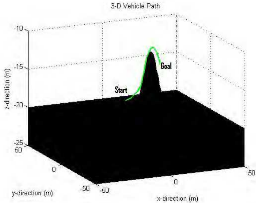
Fig. 10. The AUV kinematic model steep hill scenario.
