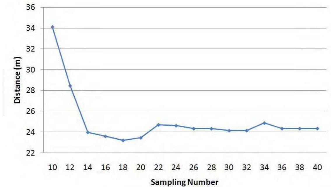
Fig. 17. The effect of sample size on path cost.
