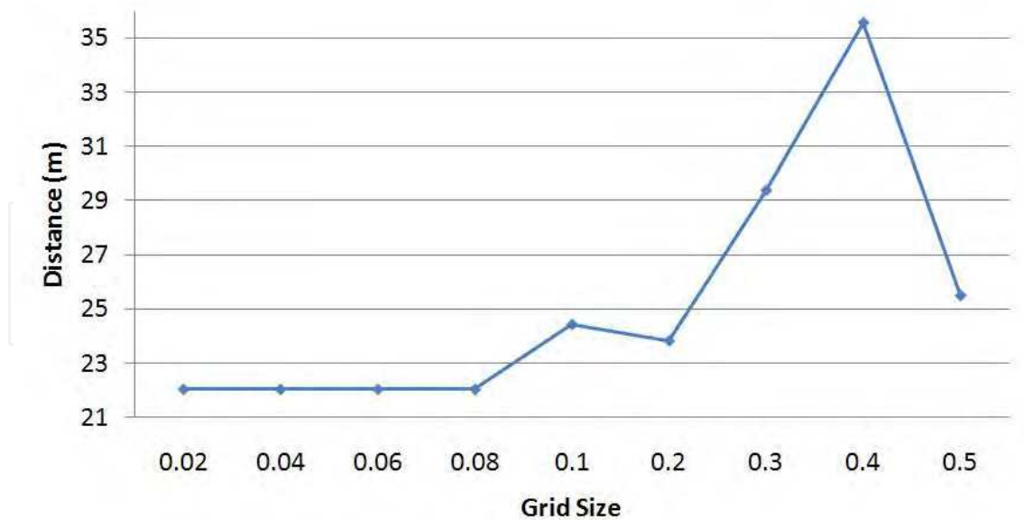
Fig. 19. The effect of grid size on path cost.
