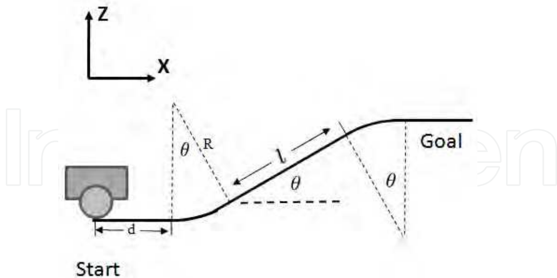
Fig. 13. The UGV steep hill parameters.
