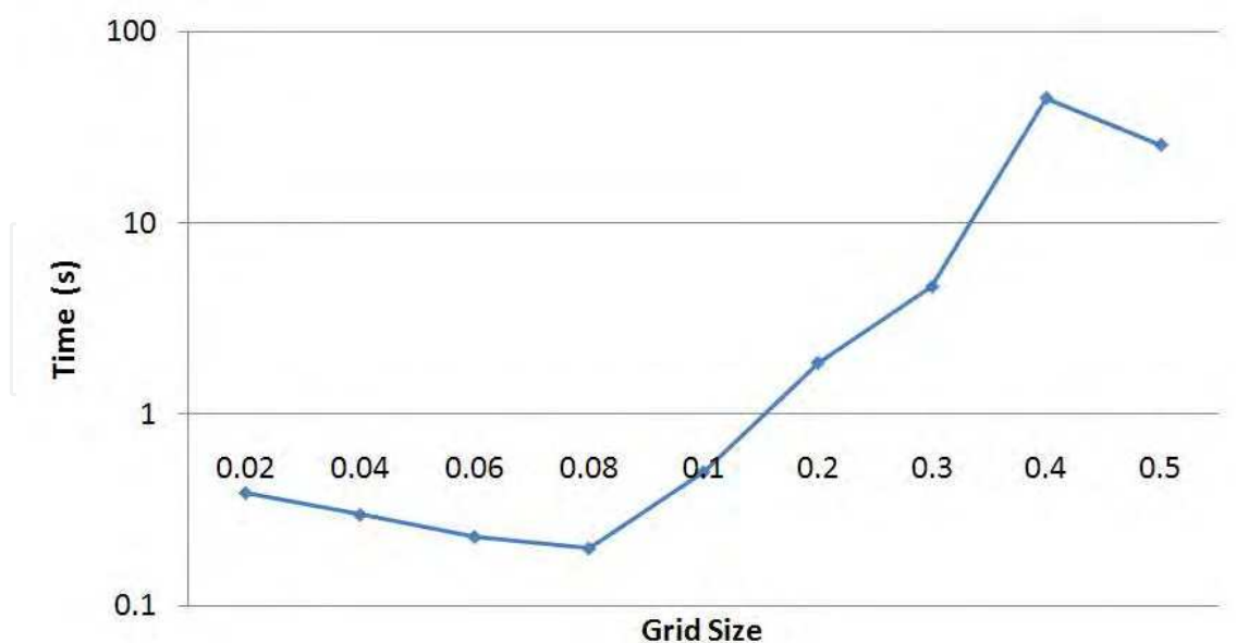
Fig. 18. The effect of grid size on computation time.
