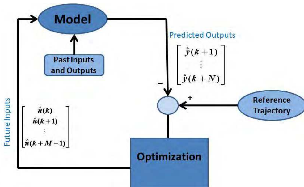
Fig. 1. The stages of the MPC algorithm.
