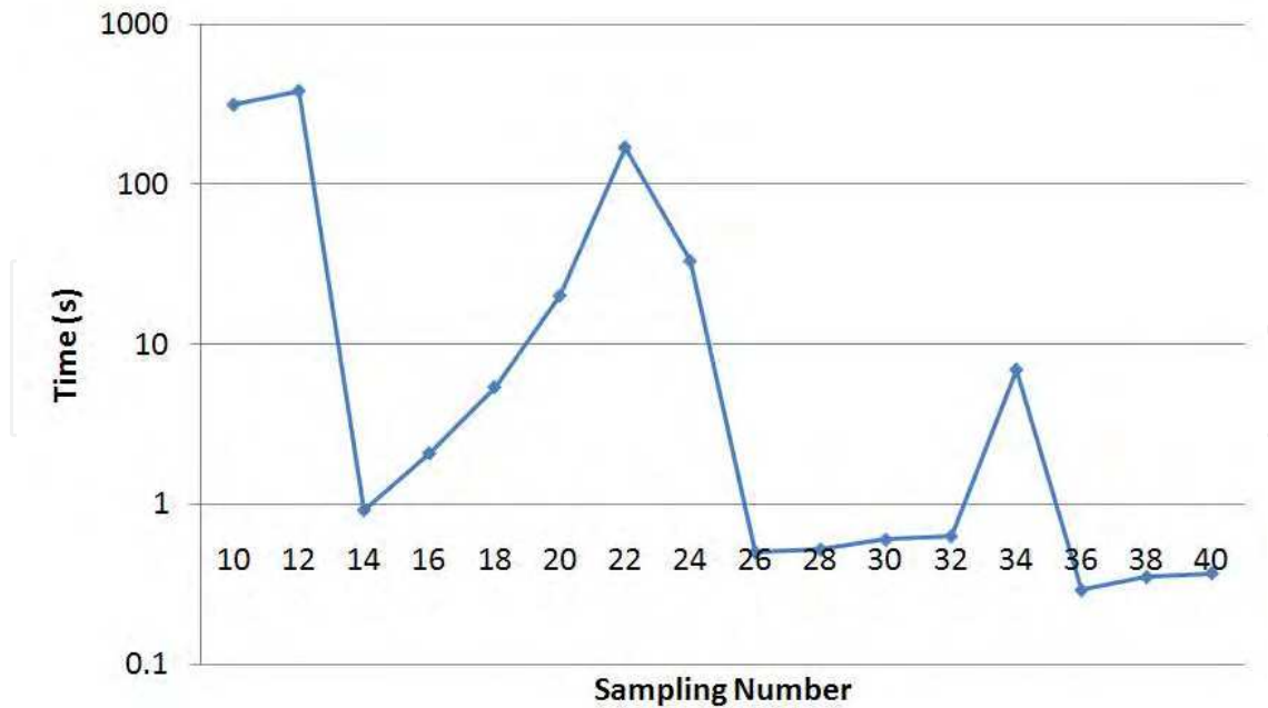
Fig. 15. The effect of sample size on computation time.
