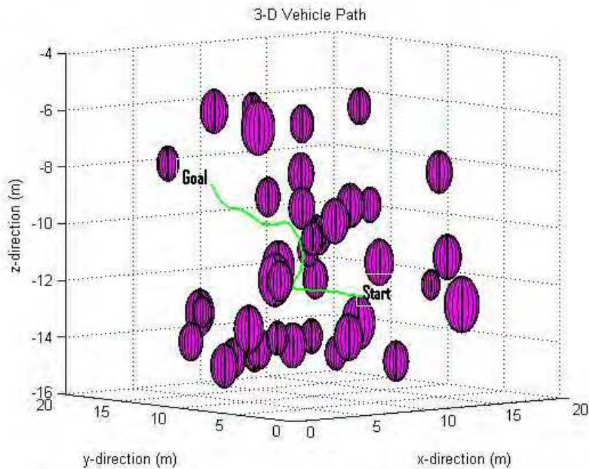
Fig. 8. A random start, goal and obstacle scenario.
