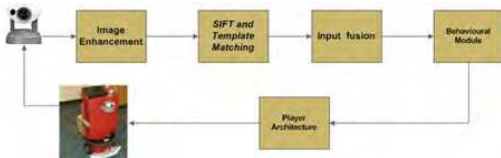
Fig. 5. Control architecture of the obstacle avoidance system.
