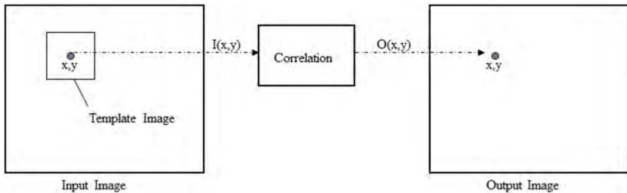
Fig. 12. Correlation technique based Template Matching.
