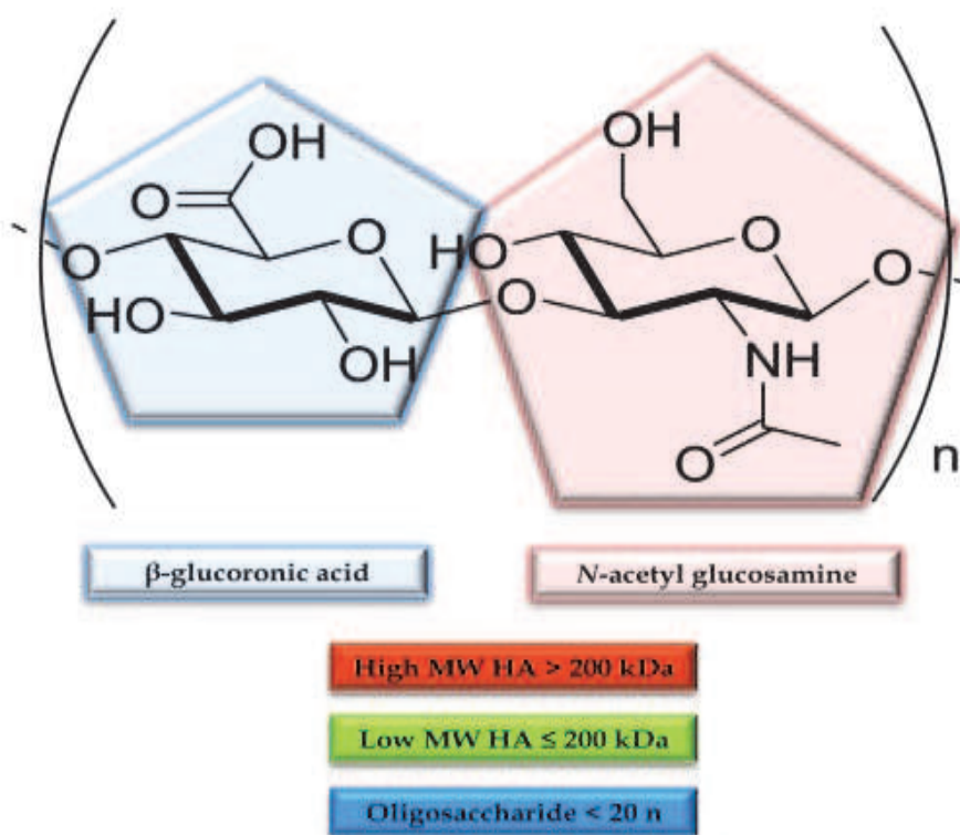
Fig. 2. HA structure and molecular weight ranges.
