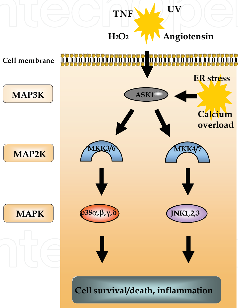
Fig. 1. ASK1, along with at least 20 other kinases belongs to the MAP3K family of enzymes. MAP3K selectively activate MAP2Ks with in turn activate members of the MAPK family. There are 7 MAP2K and 11 MAPK family members with the global MAPK family constituting 8% of the kinome. Specifically, ASK1 responds to multiple extracellular and intracellular stimuli by selectively phosphorylating MKK3/6 and/or MKK4/7 leading to the specific activation of the p38 and JNK MAPK pathways
