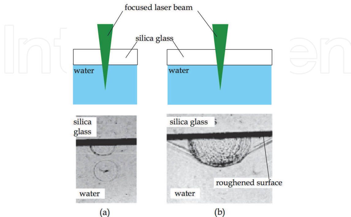
Fig. 2.2 High speed imaging of laser focus into water through silica glass plate with smooth (a) and ground surface (b). Silica glass plate was roughened by #1000 powders. Delay time of photos are 0.56 and 1.0 \mu s, respectively with a focused laser pulse of 100 mJ.
