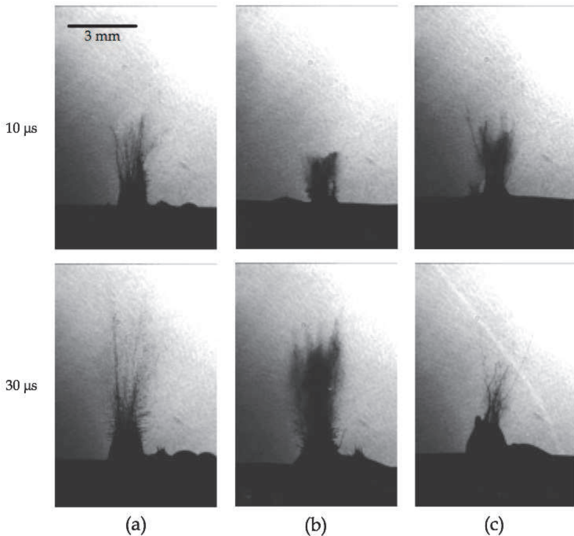
Fig. 4.7 Jet behavior of liquid specimens using assembly of Fig. 4.6. Liquid samples used are (a) : water, (b) : ethanol and (c) : vacuum oil.
