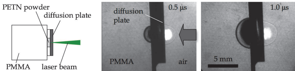
Fig. 2.6 Detonation induced stress wave in PMMA slab by pulse laser ablation of ground glass plate (diffusion plate) with surface roughness of #800 in contact with PETN high explosive powder of initial density of about 1.0 \text{ g/cm}^3 . Delay time of photographs is shown in the figure.
