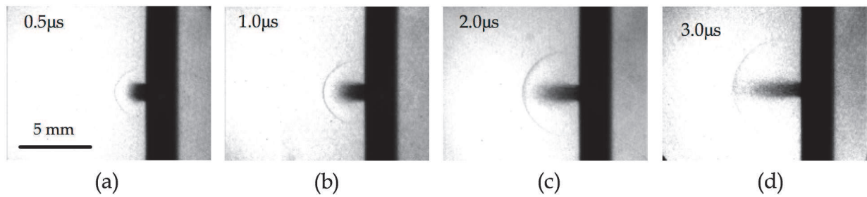
Fig. 2.3 High speed imaging record of glass fragments ejected from the ground glass surface with #240 surface roughness by pulse laser beam focused through the glass plate from right. Delay time of photographs are shown in the figure. Laser energy, focused diameter and fluence are 0.39 J, 1.8 mm, and 15.5 J/cm 2 , respectively.
