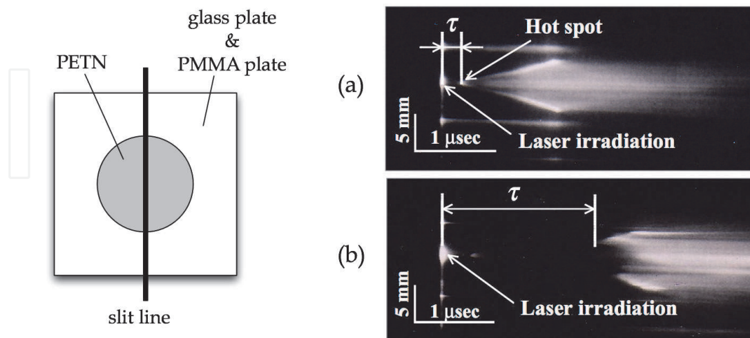
Fig. 2.7 Time sequence of PETN powder initiation experiment. Streak record of self emission by laser ablation and by reaction was obtained by a high-speed streak camera. (Imacon 790) Diffusion plate of #400 was used. Laser fluence is set to (a) 15.1 \text{ J/cm}^2 , and (b) 9.1 \text{ J/cm}^2 , respectively. Ignition delay time \tau is defined as in the figure.
