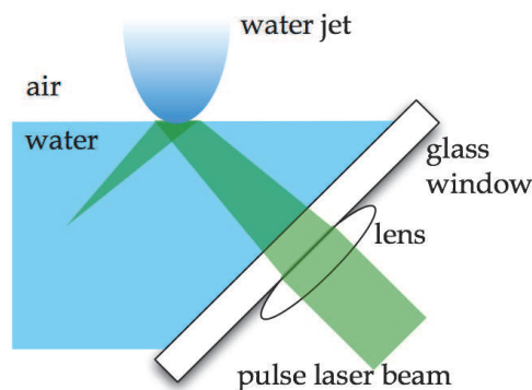
Fig. 4.1 Concept of experimental assembly for fluid experiment.
