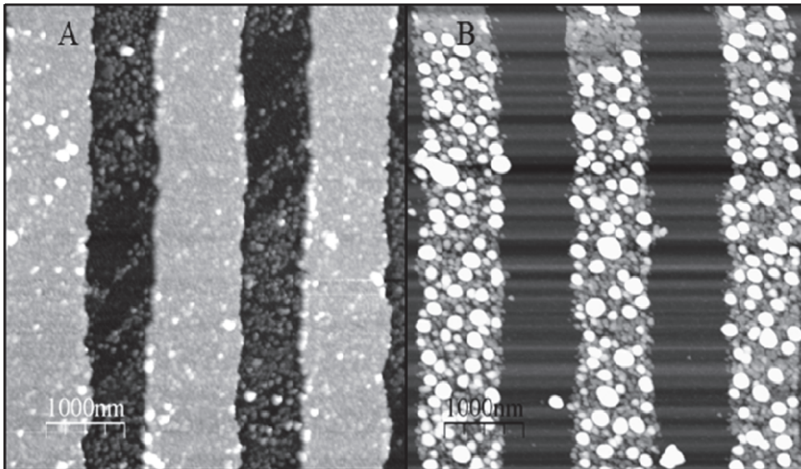
Fig. 6. Annealing effect on a lift-off patterned sample consisting of 20 nm of Ag evaporated on 70ML of Xe grating on Ti/SiO 2 /Si surface. A and B: AFM images in ambient conditions before and after annealing to 600K, respectively.
