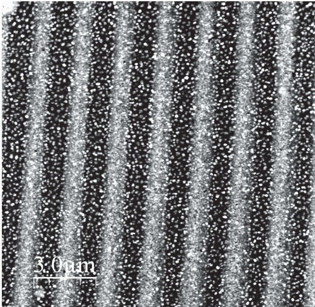
Fig. 2. AFM image of BLALP patterning of 12 nm thick layer of Au deposited on top of 10ML CO 2 buffer material on a SiO 2 /Si(100) sample at 25 K. Laser power was 14 MW/cm 2 .
