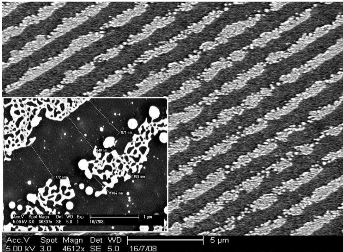
Fig. 4. SEM image of lift-off patterning of 18 nm Au on top of \text{SiO}_2/\text{Si} surface. The power of the first and second laser pulses was 12 and 9\text{MW}/\text{cm}^2 , respectively. Inset depicts the corrugated (and fragmented) texture of the resulting metal wires.
