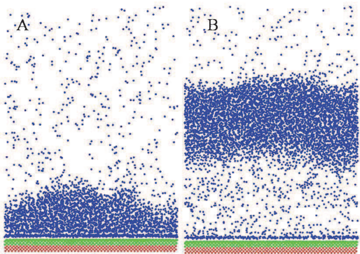
Fig. 3. Snapshots from MD simulations performed on 7744 Xe atoms adsorbed on top of Si(100) surface. A and B represent evaporative and explosive desorption while irradiating the surface by 12 and 16 MW/cm 2 pulse power, respectively. Snapshots were taken at 9.4 ns (A) and 6.6 ns (B) from the onset of the laser pulse.
