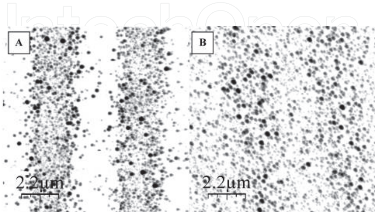
Fig. 1. AFM images of a high density gold cluster coverage grating created via BLALP scheme, evaporating 1nm of gold on top of 60ML of Xe. All images were taken at ambient environment. A) After annealing in vacuum to 300K and kept at room temperature. B) After annealing to 450K at 3K/s and quenched back to room temperature. Images are courtesy of Kerner et al., 2005.
