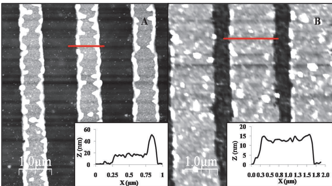
Fig. 5. AFM images of lift-off patterning procedure including line scan along the red line. A) 15 nm of Ag on top of a coverage grating formed via a 50ML Xe on \text{Ti}/\text{SiO}_2/\text{Si} surface. First and second pulse power were both of 10\text{MW}/\text{cm}^2 . B) 12 nm of Ag on top of grating produced with 70ML Xe on top of \text{Ti}/\text{SiO}_2/\text{Si} surface. Both the first and second pulses were at 14\text{MW}/\text{cm}^2 .
