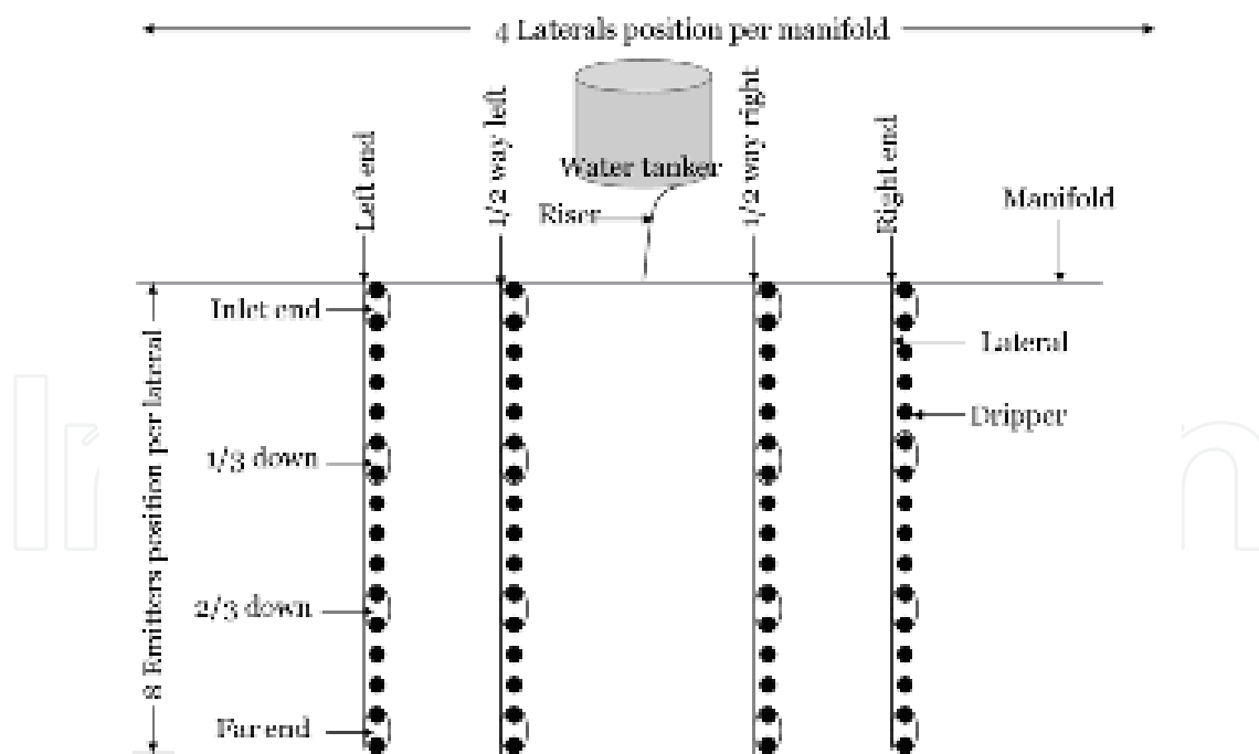
Total plot area 500 m 2 . Spacing between laterals = 0.75m and drippers = 0.3m, manifold and lateral length 20m & 25m
