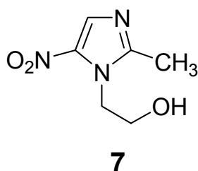
Fig. 6. Chemical structure of the antiprotozoal agent metronidazole (7).
