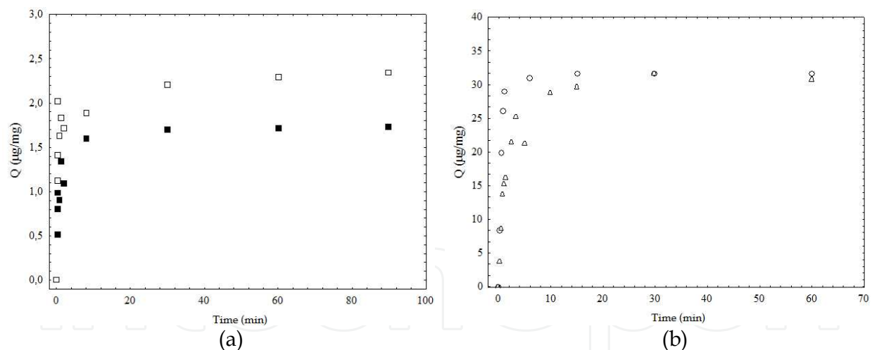
Fig. 4. Adsorption kinetics of [D-Leucine 1 ]MCYST-LR on the activated charcoals: (a) □ AC-B-F, ■ AC-A-B, and (b) ○ AC-R-G and △ AC- CS - F.
