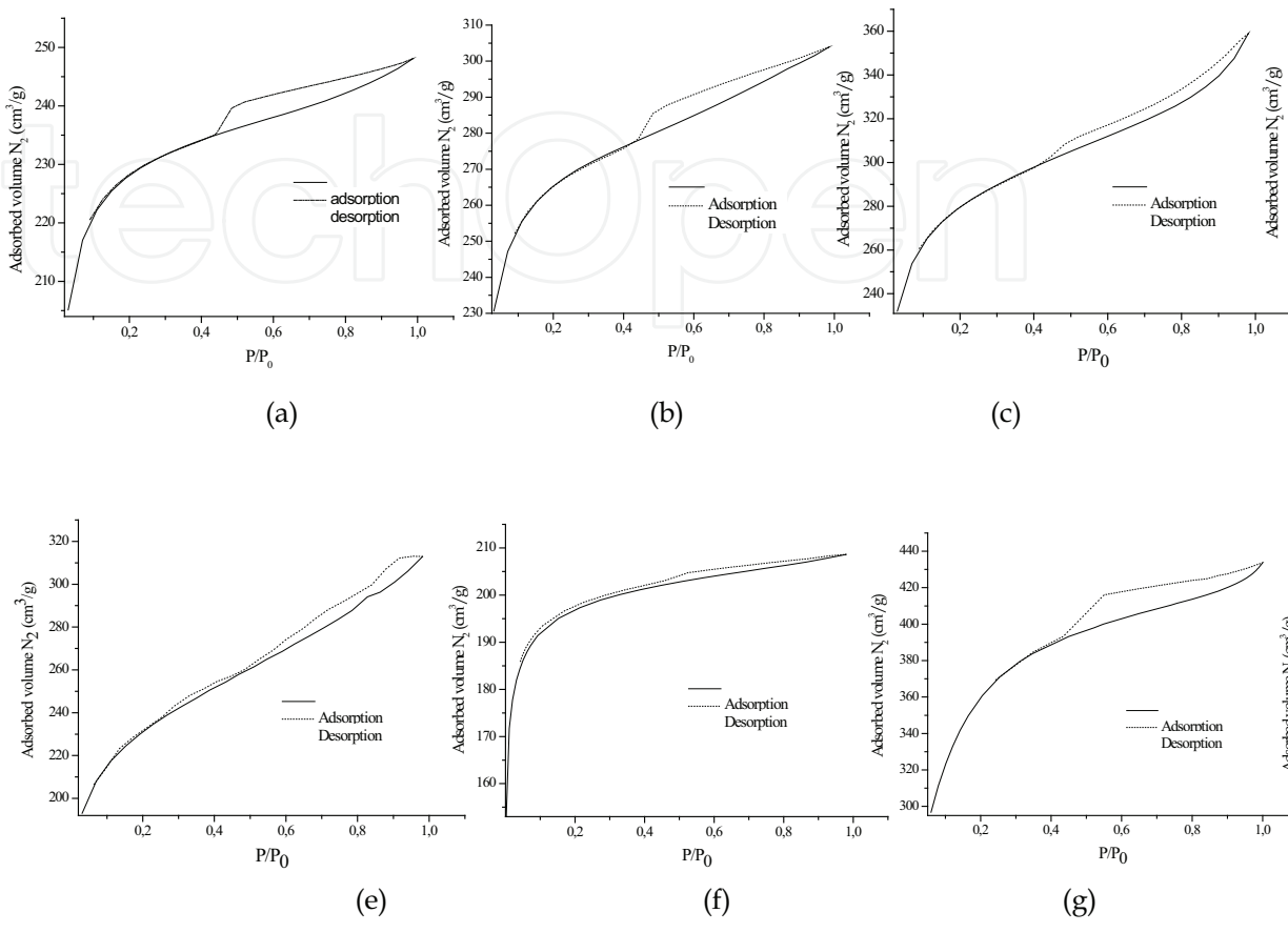
Fig. 2. Nitrogen adsorption/desorption Isothermes at -196^{\circ}\text{C} . (a) AC-A-A, (b) AC-A-B, (c) AC-A-C, (d) AC-A-D, (e) AC-B-E, (f) AC-B-F, (g) AC-R-G and (h) AC-R-H
