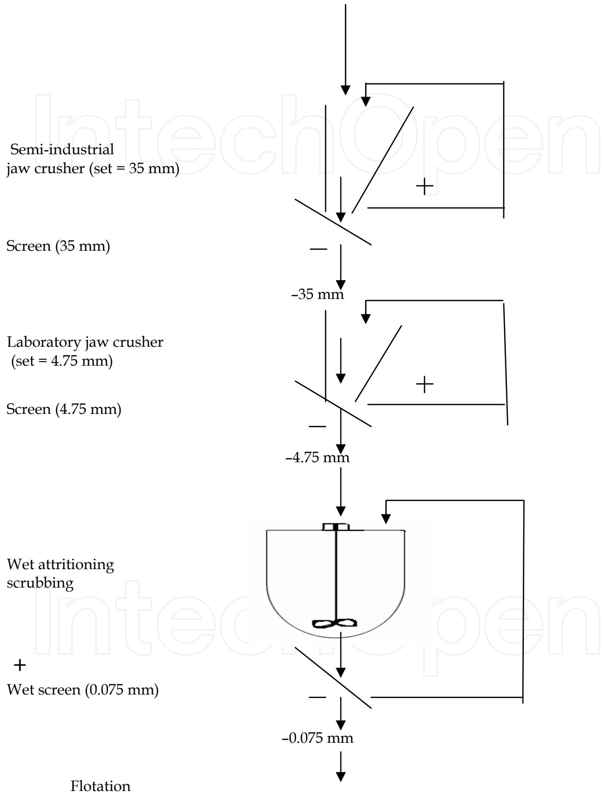
Fig. 1. Flowsheet of crushing and attritioning processes
