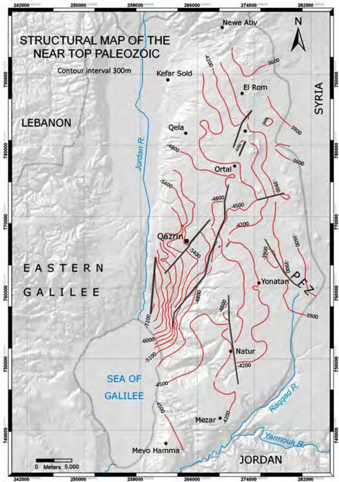
Fig. 8. Structural map of the Near Top Paleozoic Horizon (H6). After Meiler et al. , 2011. Note the western dip of the horizon from \sim 3600\text{m} at the Syrian border in the east to about -7200\text{m} at the Sea of Galilee area in the west. Major fault zones are indicated.
