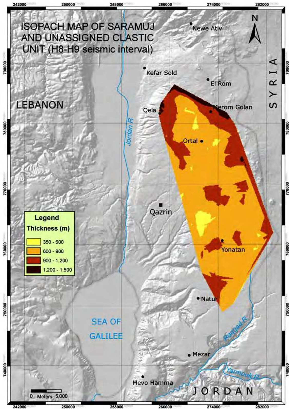
Fig. 7. Isopach map of the Sarmauj and the unassigned clastic units within the Infracambrian time span. The map represents the seismic interval calculated between H8 and H9.
