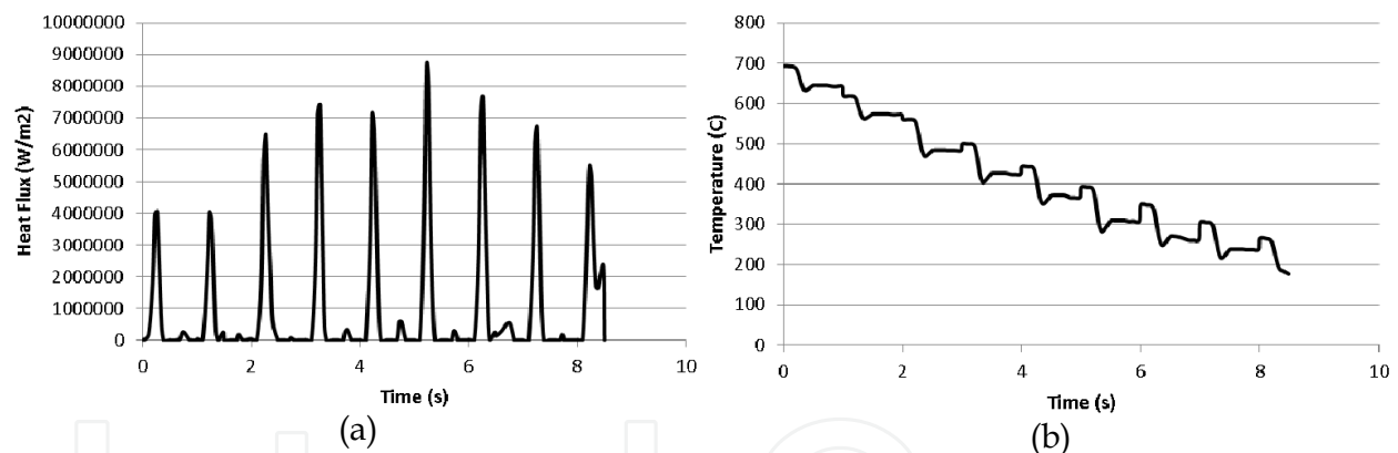
Fig. 7. Time history of cooling on a run-out table; (a) Surface heat fluxes; (b) Internal temperatures.
