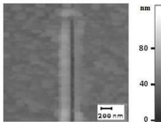
Fig. 7. Topography image of the scratch created on PMMA/glass (Sadegh Hassani et al., 2010), while the applied normal force, scanning velocity, number of scratching cycle and time of applying pressure were 3000 nN, 140 nm/s, 10 and 25 ms, respectively.
