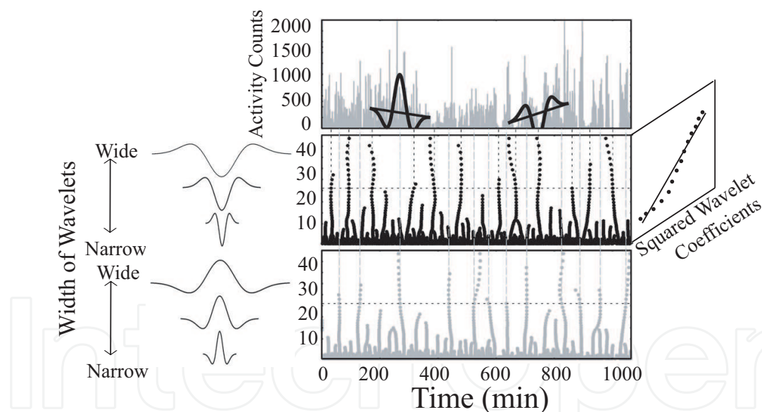
Fig. 2. Conceptual explanation of the method to obtain power-law exponents for local maxima and minima. (top) Various widths of hat-shaped wavelets are slid along the data to detect local minima (middle) and local maxima (bottom) of the wavelet coefficients. Note that the local minima and maxima appear at the transient decreases and increases of the activity, respectively. The power-law exponents are calculated from the slope of the log-log plot of squared wavelet coefficients vs. the scale for local minima and maxima. In the actual analysis, we used an integrated, rather than raw, time series and \psi(t) , i.e., the derivative of the “hat-shaped” wavelet. This yields the same power-law exponents as those obtained by the DFA method for the same local maxima and minima as obtained in this figure. Reprinted with permission from (Pan et al., 2007).
