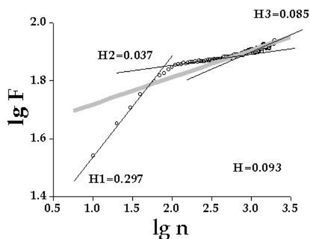
Fig. 10. Pattern of fractal dimension of the surface EMG signals with three exponents. Thick line is general exponent, thin lines are local exponents. H is general Hurst index; H1 , H2 , H3 are values of local Hurst indices.
