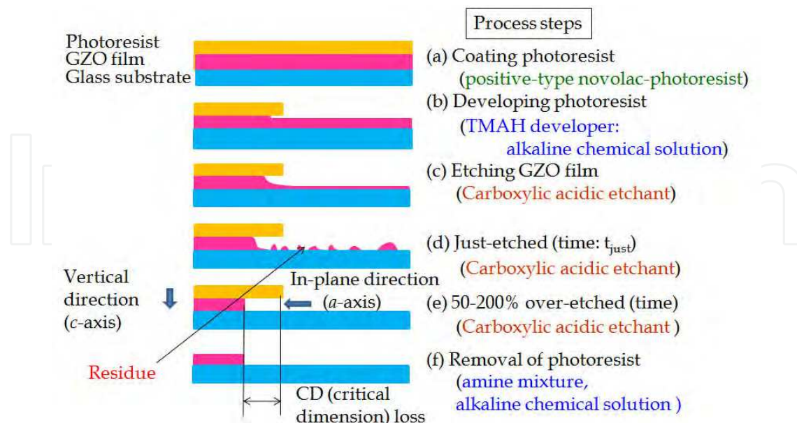
Fig. 15. Process flow for patterning GZO films using wet-chemical etching techniques
