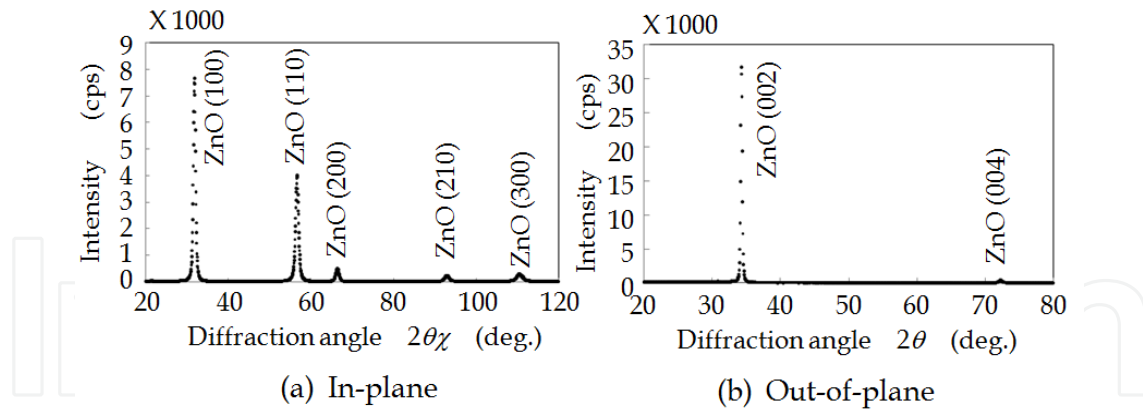
Fig. 2. Typical XRD profile of a 150 nm thick GZO film prepared at 180 °C using dc MS.
