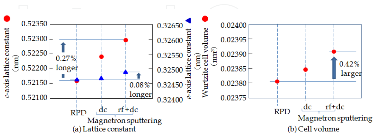
Fig. 4. Comparison of the a -axis, c -axis lattice constants and the unit cell volumes in crystalline ZnO-based wurtzite structures of films prepared using dc MS, rf+dc MS and RPD (Yamamoto, N. et al 2010).
