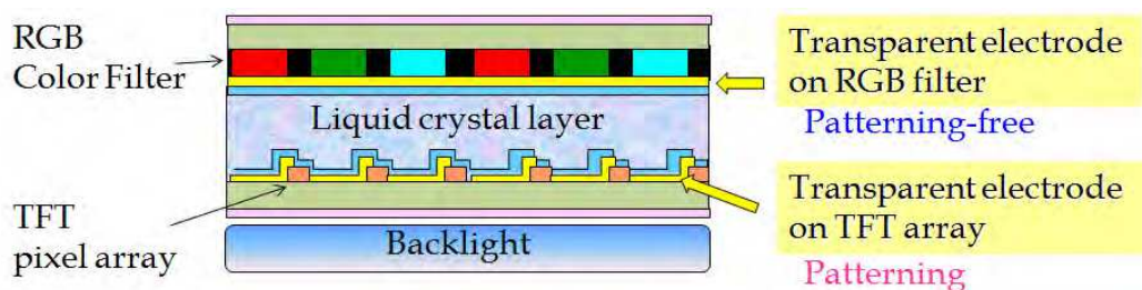
Fig. 10. Schematic cross-sectional view of an LCD.
