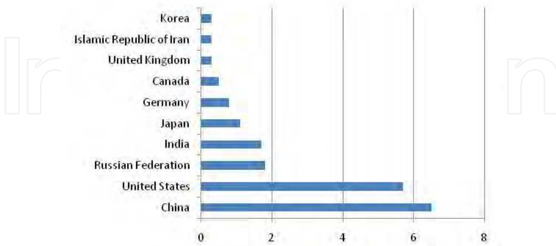
Fig. 2. Top 10 emitting countries in 2008 (Gt CO 2 ). Source: IEA, 2010.
