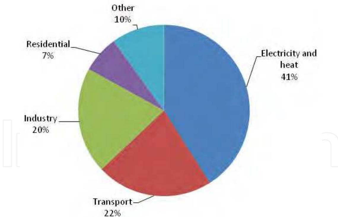
Fig. 3. World CO 2 emissions by sector in 2008. Source: IEA, 2010.
