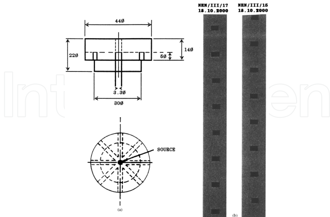
Fig. 12. (a) Specially designed autoradiography gadget; b) developed autoradiography film of the sources.
