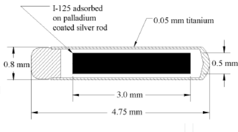
Fig. 10. Assembly of laser welded ^{125}\text{I} seed
