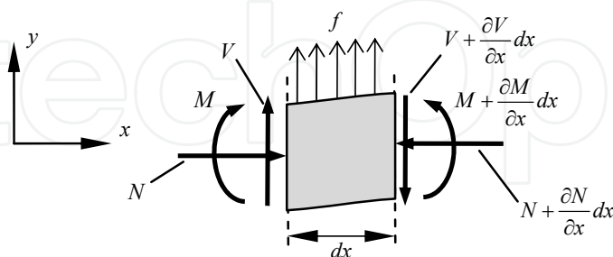
Fig. 2. Free-body diagram of Euler-Bernoulli beam segment
