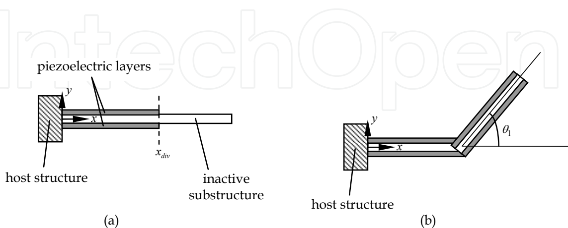
Fig. 5. (a) Layout of bimorph structure with partial piezoelectric layer coverage. (b) Layout of bimorph structure with a variable-angle bend at half its overall length.
