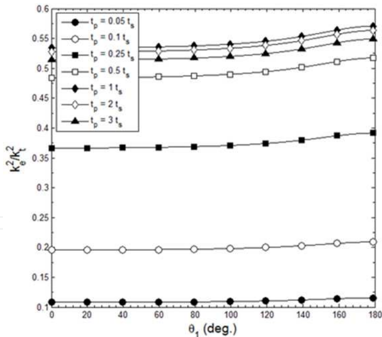
Fig. 10. Variation in coupling coefficient ratio with respect to center joint angle and layer thickness ratio.
