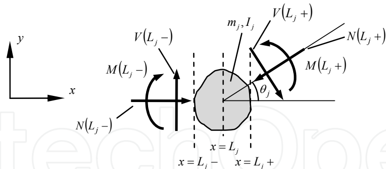
Fig. 3. Forces and moments on a lumped mass located at x = L_j .
