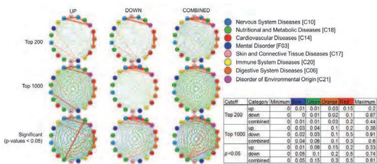
Fig. 3. DRNs for expression data for the three cutoff levels (top 200, top 1000, and significance with p -value < 0.05 ) and three expression categories (up-regulated, down-regulated, and combined). Disease nodes are color coded to show grouping of diseases based on MeSH classification. Edges are color coded according to increasing strength of disease association. Values for the color scale are listed in the inserted table.
