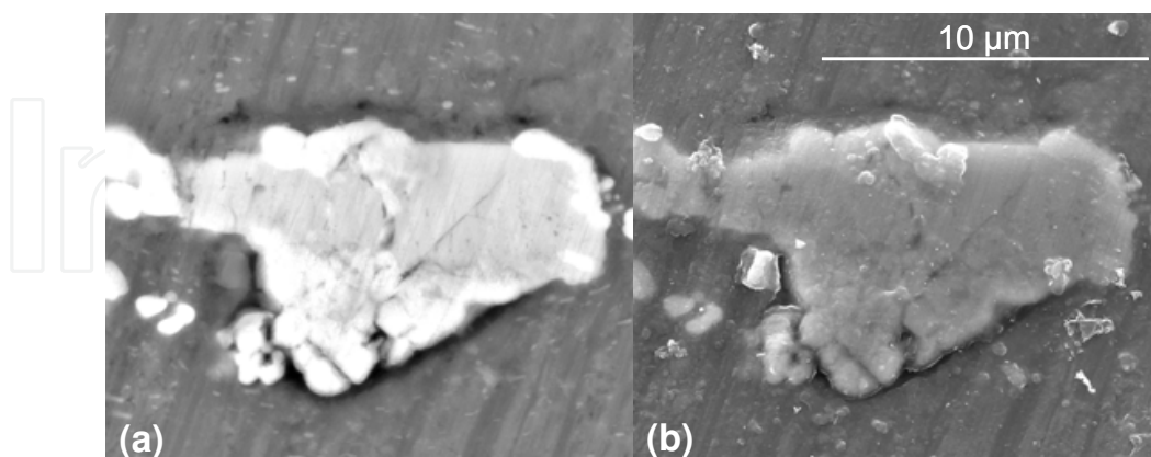
Fig. 5. (a) backscattered and (b) secondary electron images of an IM particle with compositional domains. Corroded in 0.1 M NaCl for 30 minutes at room temperature
