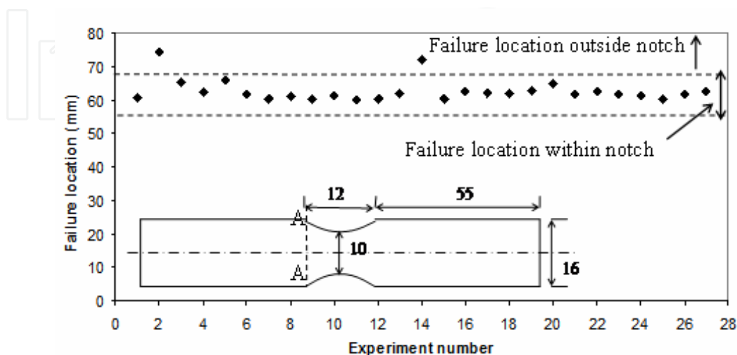
Fig. 13. Failure location in aluminium TWB (Abhishek et al., 2011)
