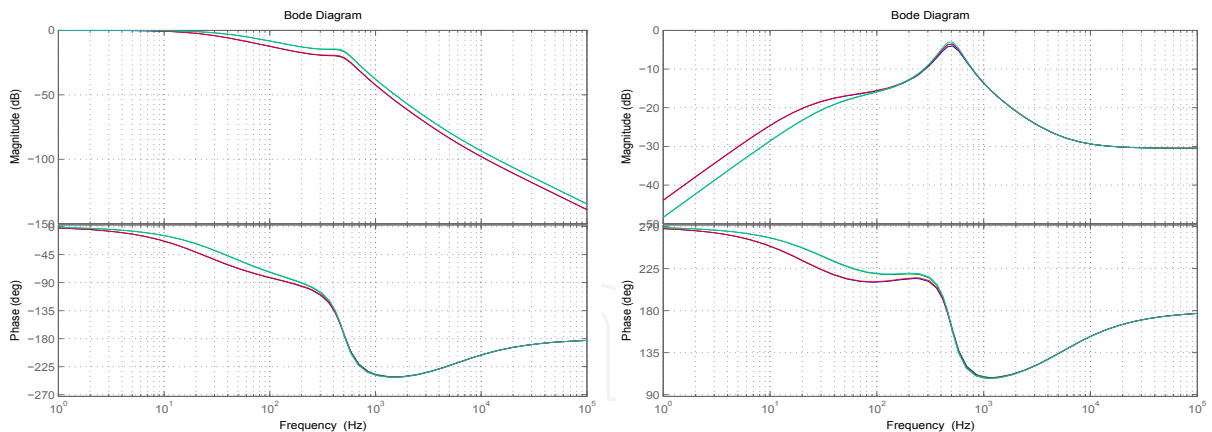
(a) Bode plot of closed loop transfer function from reference to output.
