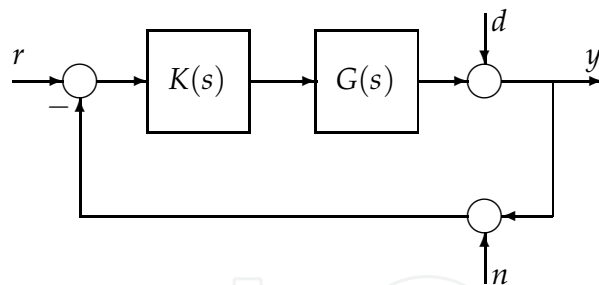
Fig. 1. One degree of freedom feedback control system.
