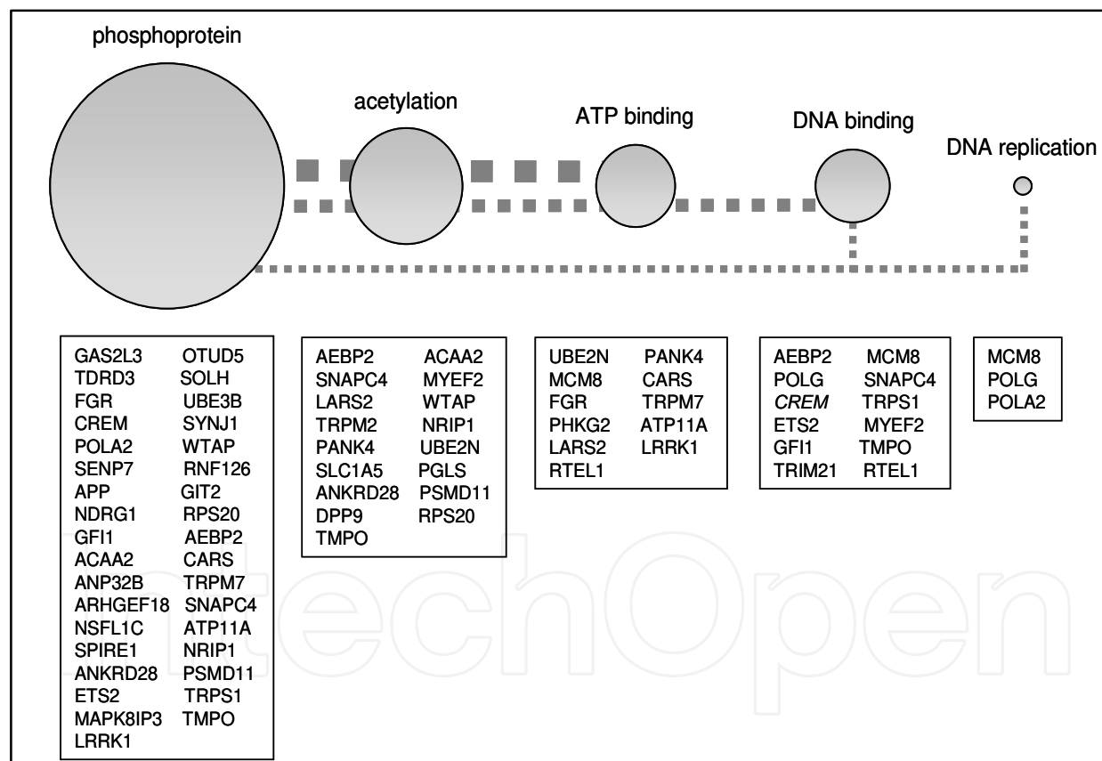
Fig. 3. Genes regulated in common by Survivin and LSC. The 76 genes up-regulated or down regulated by Survivin and LSC were functionally classified by DAVID software. The size of each circle represents the number of genes involved in each functional categories and the thickness of the line indicates the number of genes shared with any function. Functional classification was performed based on Swissprot Keywords. Genes annotated in each functional category are shown in the text box.
