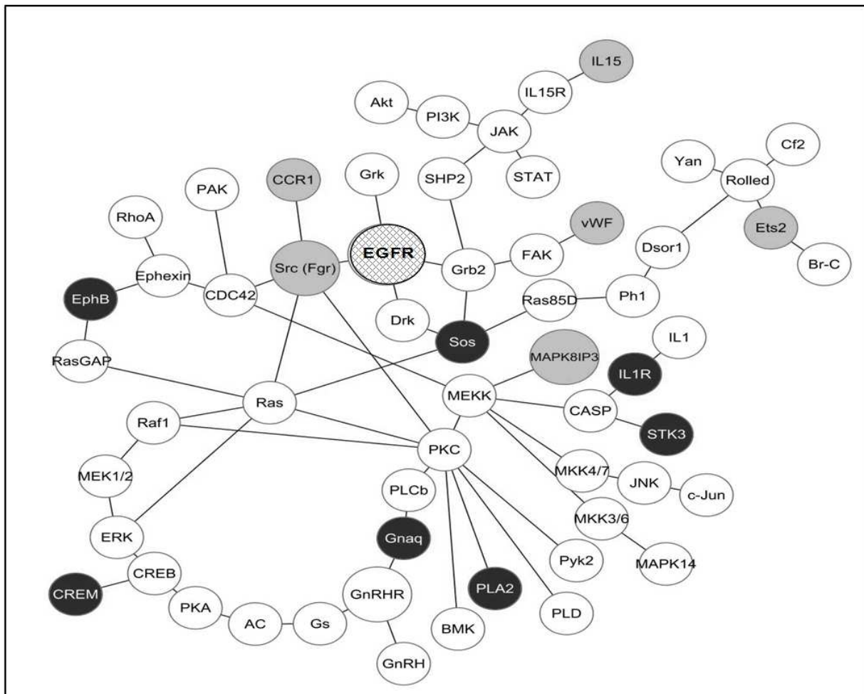
Fig. 4. Genes regulated by Survivin in ITD-Flt3 + KSL cells and deregulated in LSC are mapped on a functional signaling network associated with the epidermal growth factor receptor signaling pathway. Epidermal growth factor receptor signaling pathway (EGFR) is significantly enriched in the shared genes associated with LSC and Survivin signaling by pathway enrichment analysis in KEGG and Gene Ontology databases. Our analysis shows that 13 molecules shared by LSC and Survivin signaling are mapped on a functional signaling network associated with EGFR. The network was created based on the KEGG database using Cytoscape software. Gray and black circle represents down regulation and up regulation by Survivin gene deletion, respectively. The hatched circle shows EGFR.
