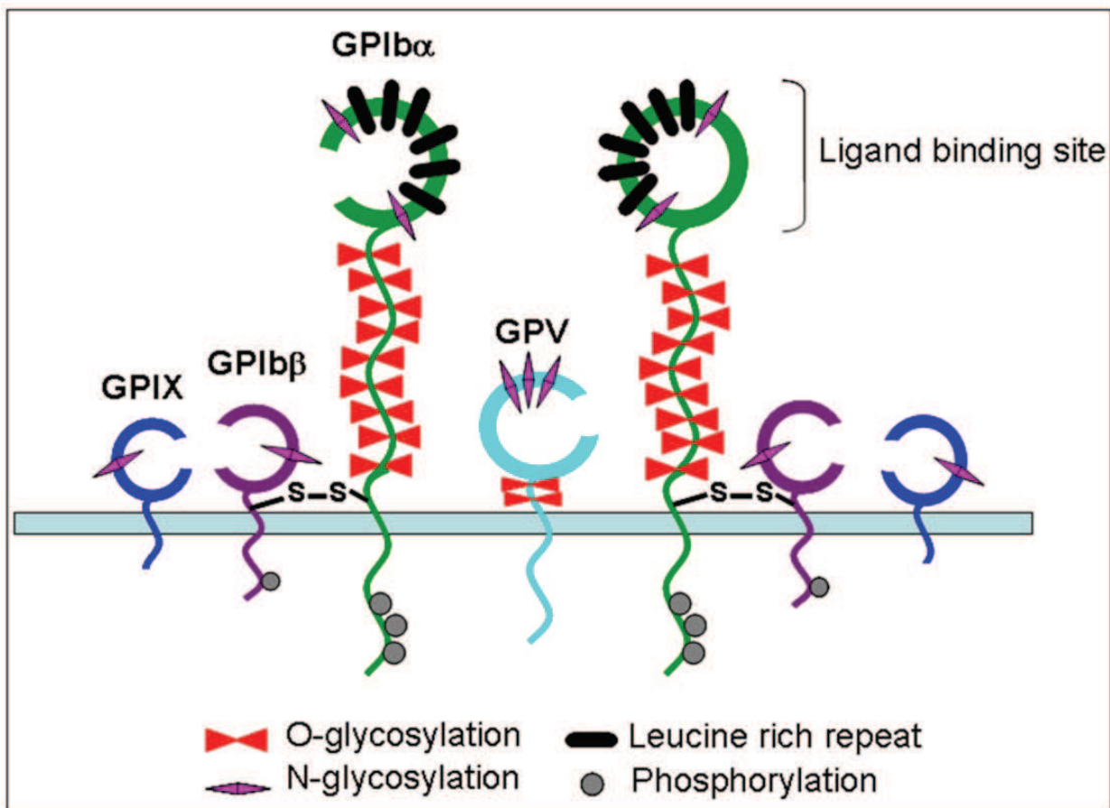
Fig. 1. GPIb-IX-V complex
