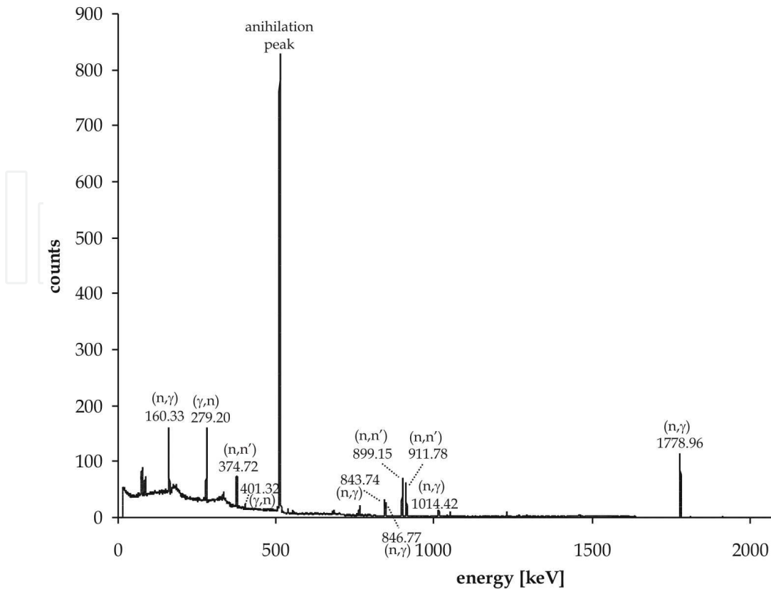
Fig. 4.6. The typical energy spectrum of gammas emitted by a medical linac accessory. The notation near the peaks is as in Figure 4.3.
