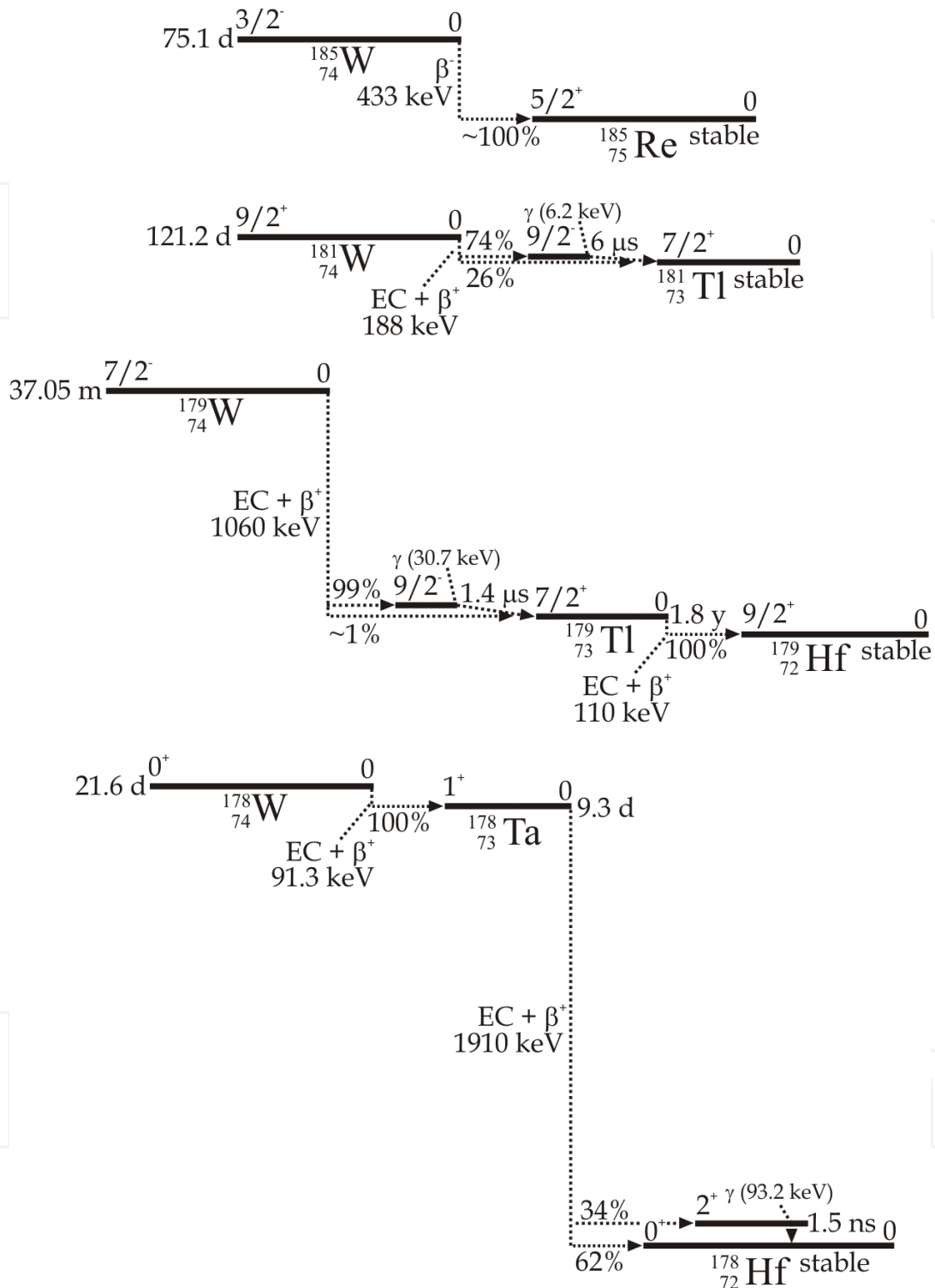
Fig. 4.10. Decay schemes of the ^{178}\text{W} , ^{179}\text{W} , ^{181}\text{W} and ^{185}\text{W} nuclei originating from photonuclear or electronuclear reactions. The gammas from the decays of these tungsten radioisotopes are difficult to identify by the gamma spectroscopy because of relatively low energy. The peaks from these gammas are not visible in the spectrum measured under the accelerator head contrary to the gammas from the decay of ^{187}\text{W} (see Figure 4.3). Low-energy peaks from decays of nuclei can be concealed among peaks from scattered radiation.
