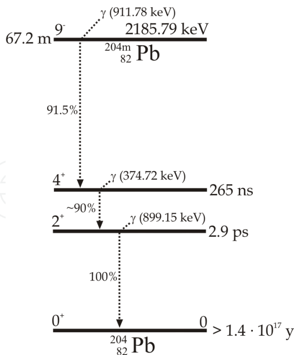
Fig. 5.5. Decay scheme of the ^{204m}\text{Pb} state. The peaks at 374.72 keV, 899.15 keV and of 911.78 keV are visible in the spectrum of gammas emitted by the accessory of a medical linac (Figure 4.6).
