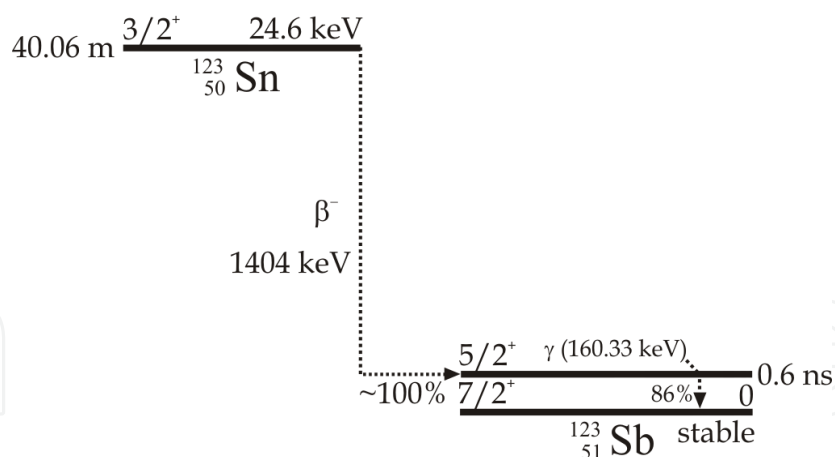
Fig. 5.4. Decay scheme of the ^{123}\text{Sn} nucleus.
