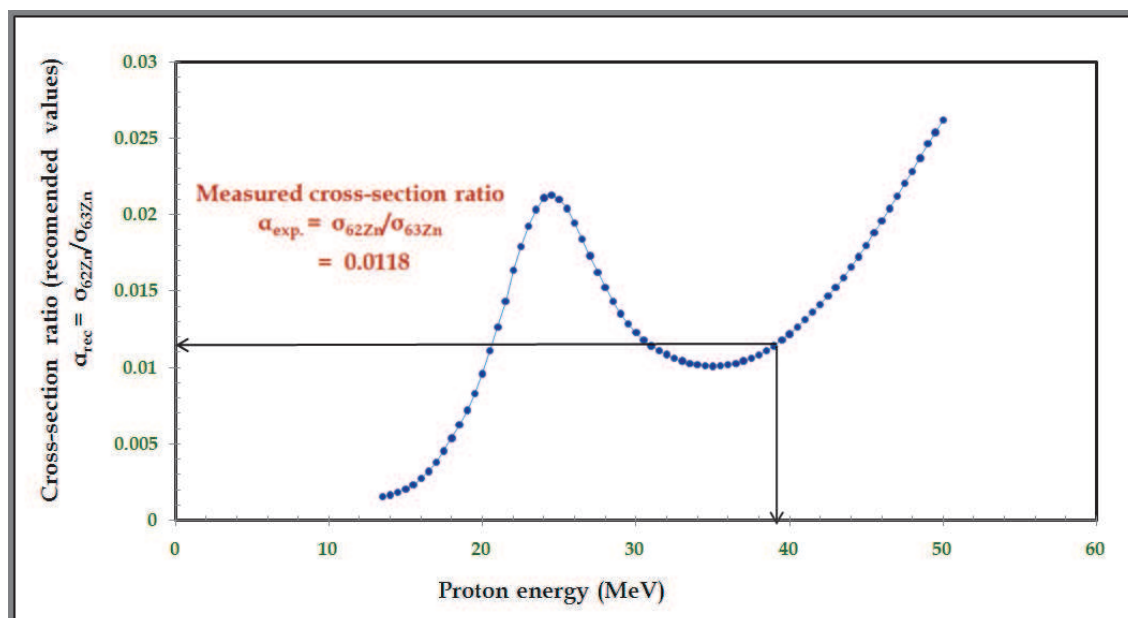
Fig. 4. The energy calibration for the Proton beam using the \alpha_{exp} ratio for \sigma_{62Zn} and \sigma_{63Zn}
