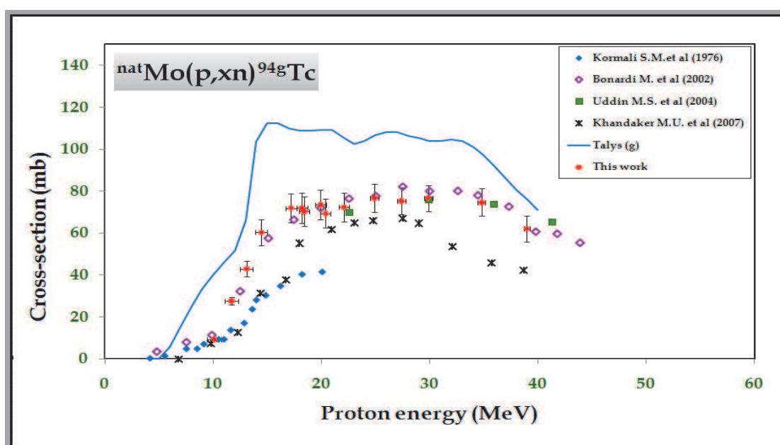
Fig. 9. Excitation function of the ^{nat}\text{Mo}(p,x)^{94g}\text{Tc} reaction (full red dots) compared to some previously published results and the TALYS code calculations (curve).
