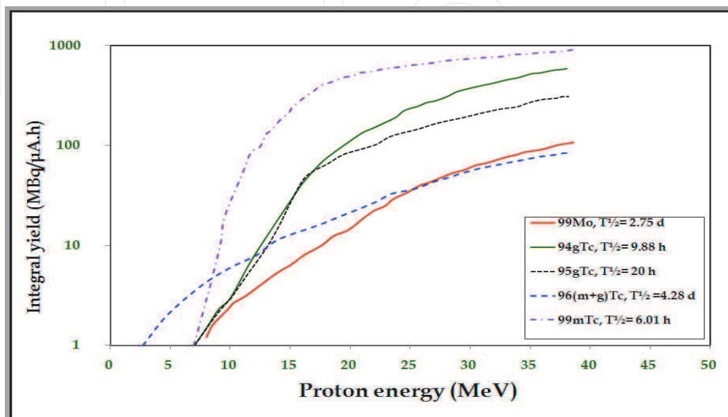
Fig. 13. Integral Yields for the ^{nat}\text{Mo}(p,x)^{99}\text{Mo} , ^{94g} , ^{95g} , ^{96(m+g)} , ^{99m}\text{Tc} nuclear reactions calculated from the excitation functions measured in this work.
