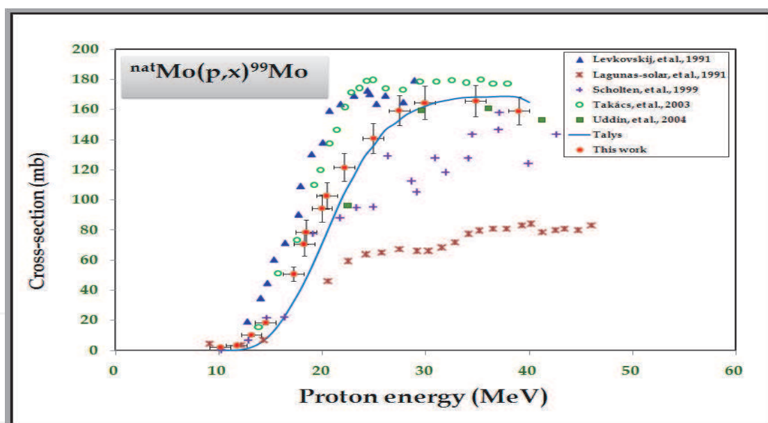
Fig. 8. Excitation function of the ^{nat}\text{Mo}(p,x)^{99}\text{Mo} reaction (full red dots with vertical and horizontal error bars) compared to some previously published results and the TALYS code calculations (curve).
