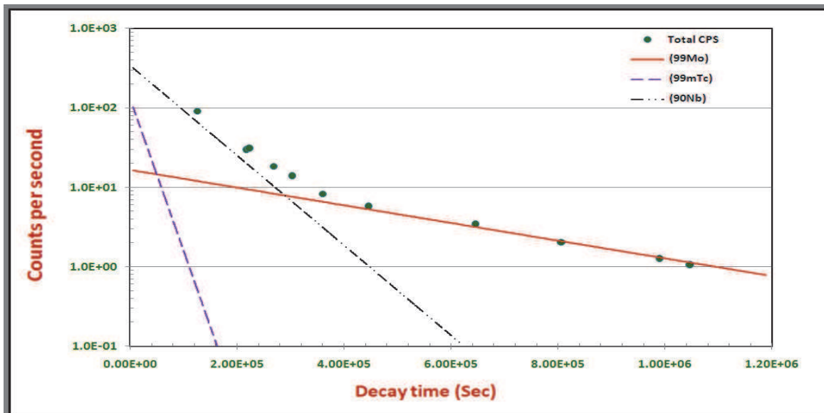
Fig. 7. Resolving the 140 keV \gamma -line which produced from three different radioisotopes 99 Mo, 99m Tc and 90 Nb
