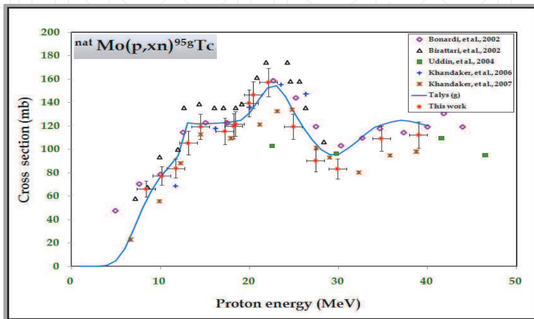
Fig. 10. Excitation function of the {}^{\text{nat}}\text{Mo}(p,x){}^{95\text{g}}\text{Tc} reaction compared to some previously published results and the TALYS code calculations.
