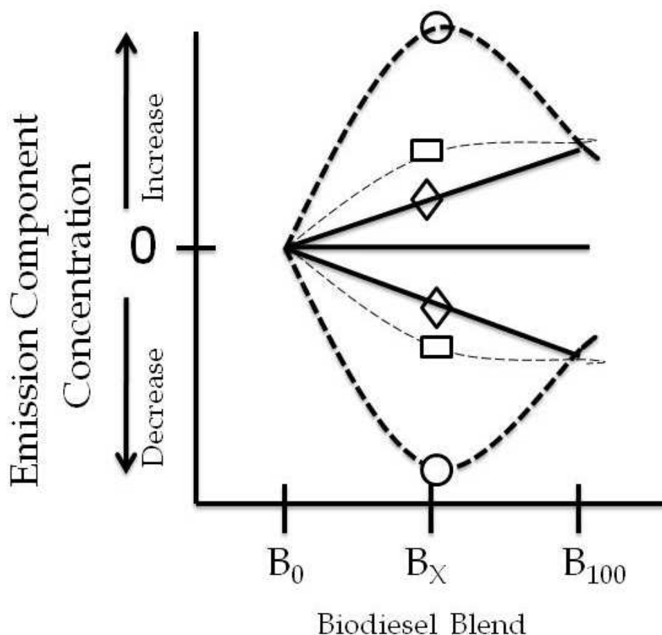
Fig. 1. Theoretical changes in an emission component as the proportion of biodiesel changes from 0 ( B_0 ) to 100 ( B_{100} )%. Linear changes are reflected by straight lines and diamonds, concave and convex changes are reflected by dashed lines and circles, and sigmoidal changes are reflected by dashed lines and rectangles.
