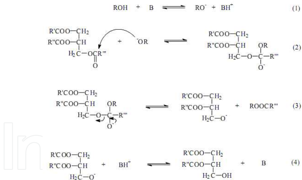
Fig. 11. Mechanism of the base-catalyzed transesterification of vegetable oils.
