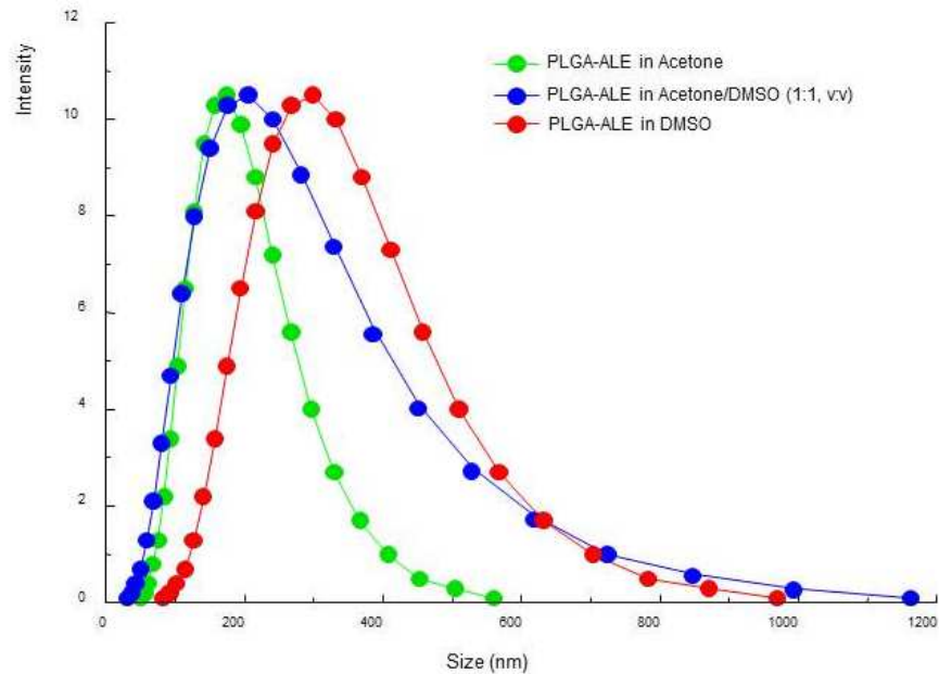
Fig. 4. Size distribution patterns of PLGA-ALE NP prepared using different organic phases (adapted from [31]).
