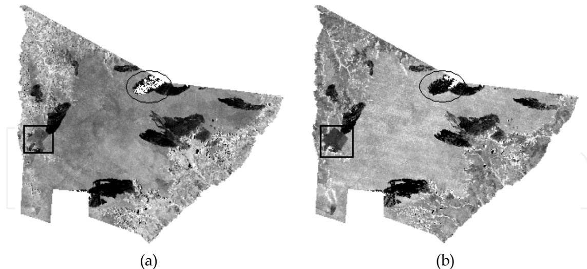
Fig. 4. Near infrared band - IR (a) and NDVI image (b)
