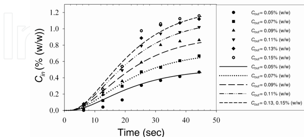
Fig. 10. Comparison of the experimental (e0.05, e0.07, e0.09, e0.11, e0.13 and e0.15) and theoretical data (s0.05, s0.07, s0.09, s0.11, s0.13 and s0.15) of the droplet-based microextraction kinetics
