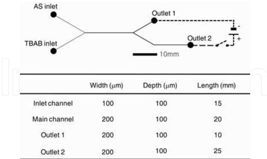
Fig. 7. Y-branched microfluidic device design for the droplet transport experiment
