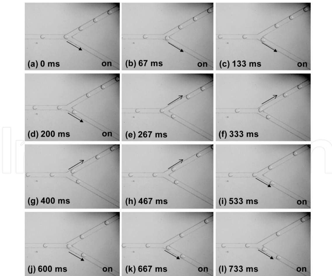
Fig. 8. Transport of a droplet into the desired channel by the application of electric pulses
