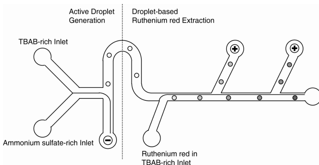
Fig. 12. The schematic diagram of the microfluidic system for microextraction control. Droplets can be moved to one of the two branched channels by applying an electric pulse after cessation of microextraction.
