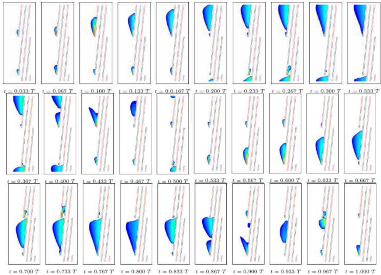
Fig. 12. Rotating blade cavitation on a two-blade inducer ( \sigma=0.258 and \Phi=0.039 ). Calculations using RNG \kappa - \epsilon modified turbulence model
