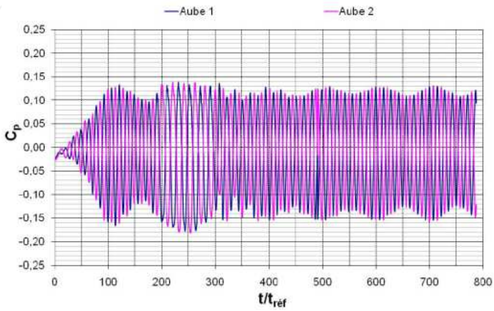
(a) Two-blade cascade
