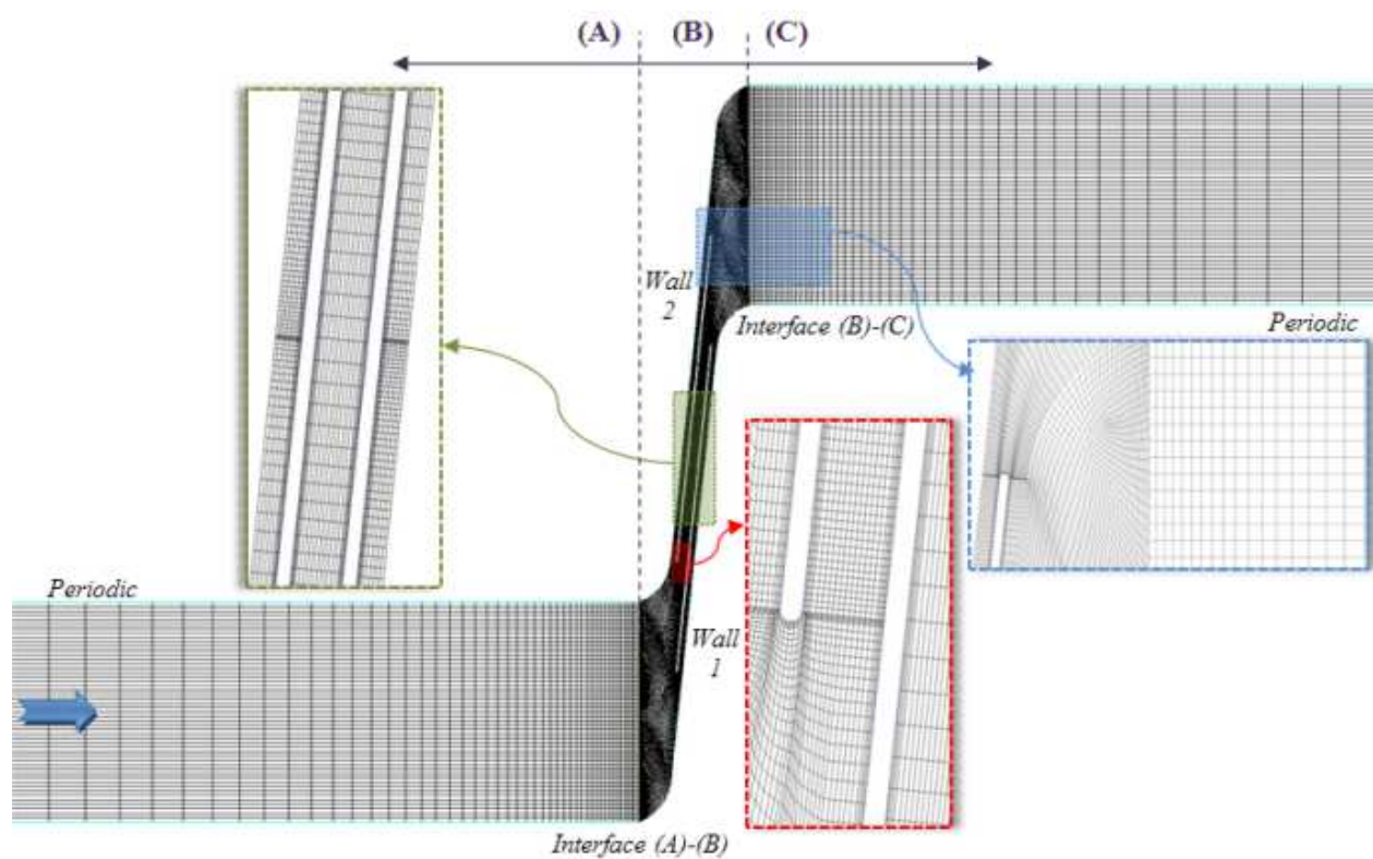
Fig. 6. Blades cascades corresponding to the inducers studied, see Fig. 1
