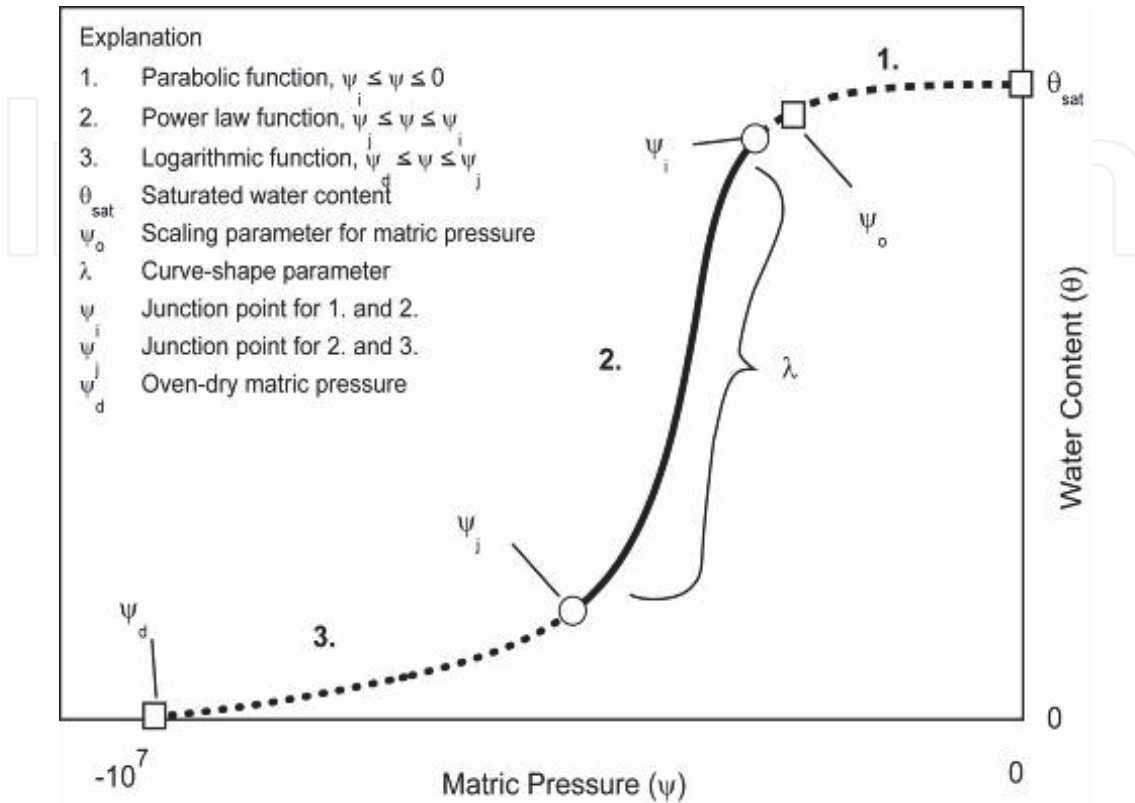
Fig. 2. Example of water-retention ( \theta(\psi) ) curve showing the components of the curve-fit model developed by Rossi and Nimmo (1994).
