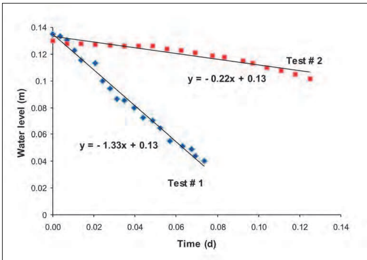
Fig. 6. Measured water level versus time during tests # 1 and #2 at the Altamura site.
