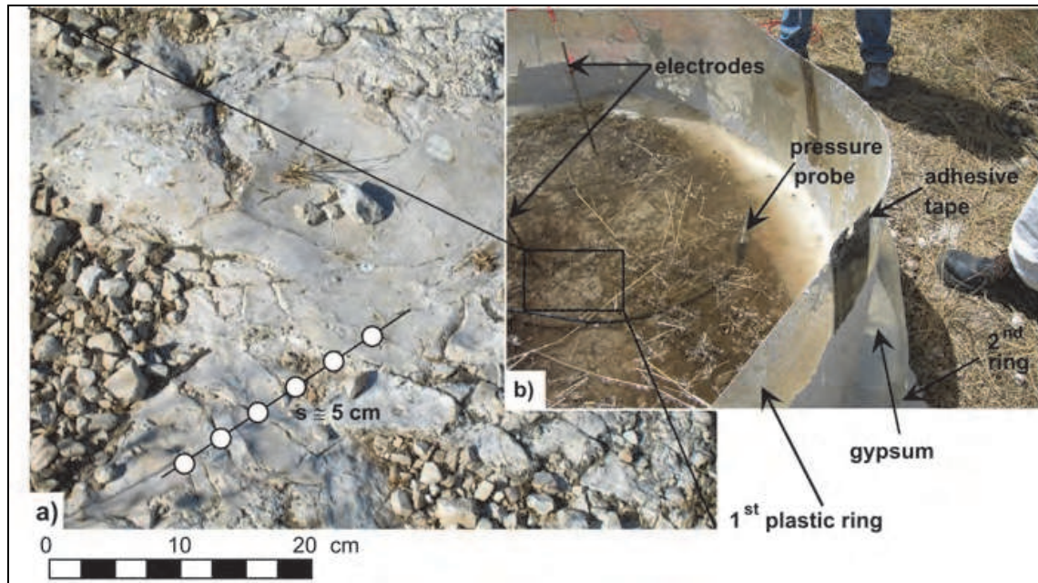
Fig. 2. Test # 1 at the Altamura site: a) fractured limestone with visible fractures of about 5 cm of spacing ( s ); b) plastic ring infiltrometer resting directly on the ground and sealed with gypsum by using a second ring.
