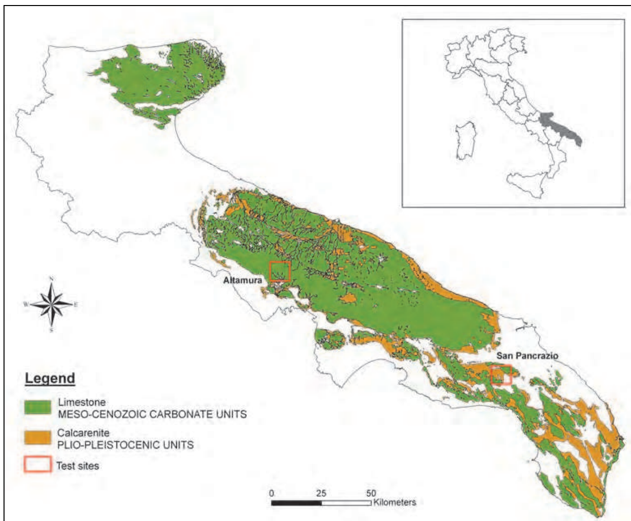
Fig. 1. Schematic geological map of the Puglia region.
