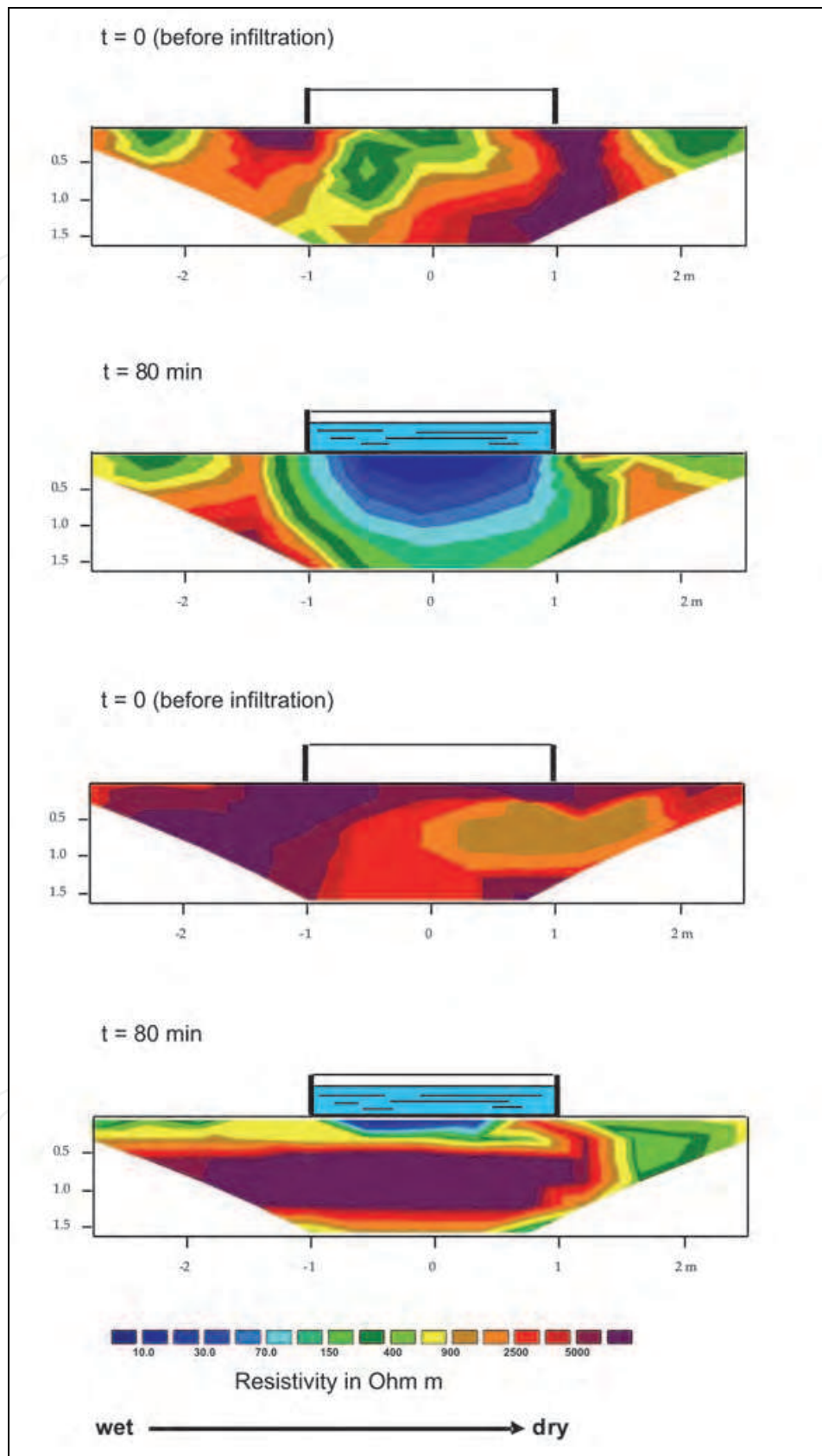
Fig. 8. Electrical resistivity profiles during test # 1 and # 2, before ( t = 0 min) and during ( t = 80 min) water infiltration tests at the Altamura site.
