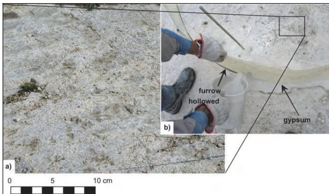
Fig. 3. Test # 2 at the Altamura site: a) limestone without visible fractures; b) plastic ring infiltrometer installed into a thin (2 cm) furrow hollowed in the limestone and sealed with gypsum.
