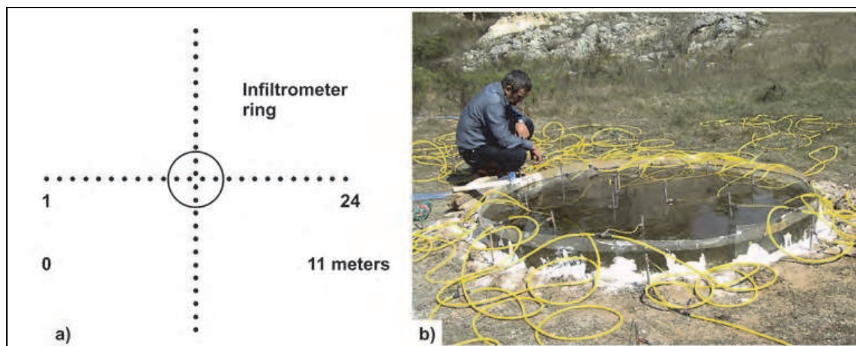
Fig. 5. Test at the San Pancrazio site: a) scheme of electrode array; b) detail of field installation of electrodes.
