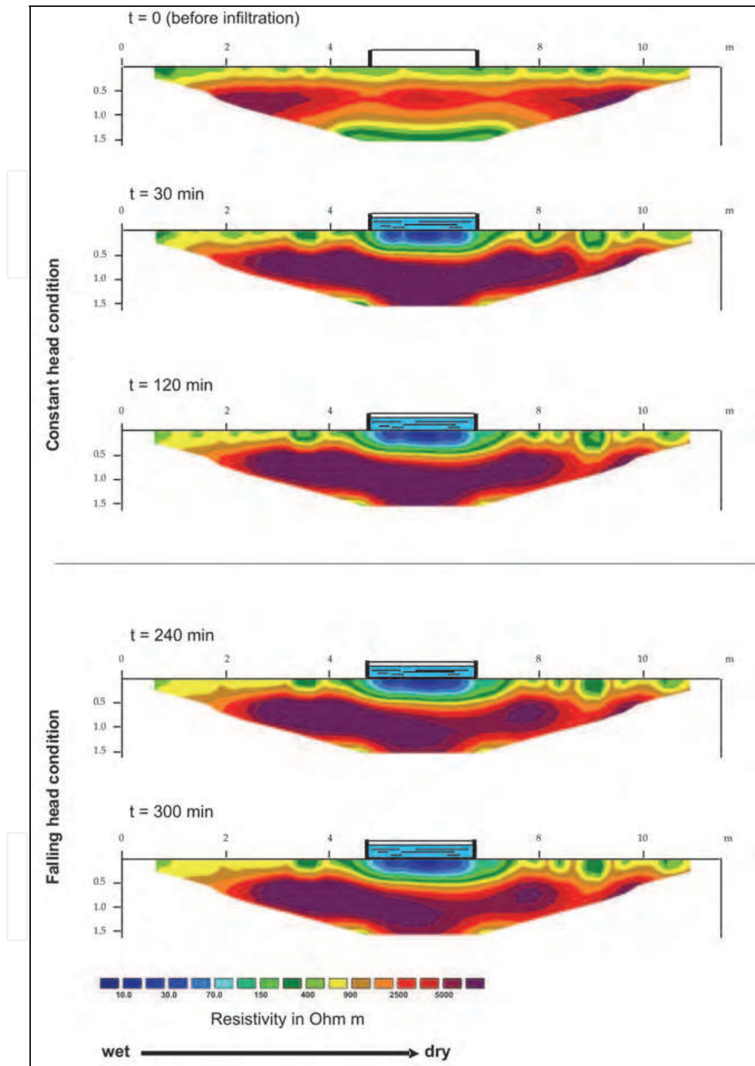
Fig. 10. Electrical resistivity profiles during infiltration test at the San Pancrazio site - profile 1.
