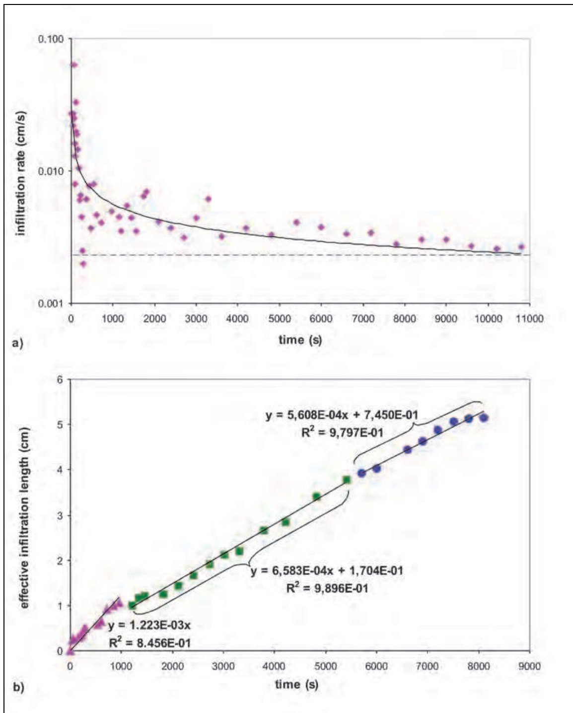
Fig. 9. Test at the San Pancrazio site: a) constant head infiltration test – infiltration rate versus time; b) falling head infiltration test – effective infiltration length versus time.
