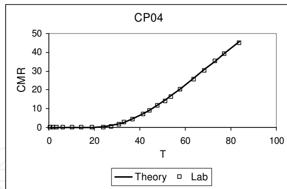
Fig. 15. Zinc cumulative mass ratio curve (CP04).
