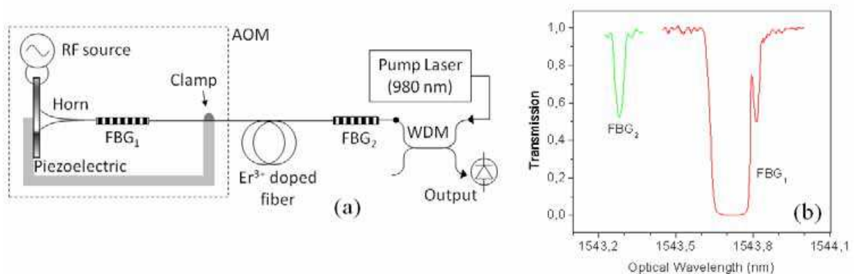
Fig. 12. (a) Laser setup, the dashed line defines the acousto-optic modulator. (b) Transmission spectra of the two fiber Bragg gratings
