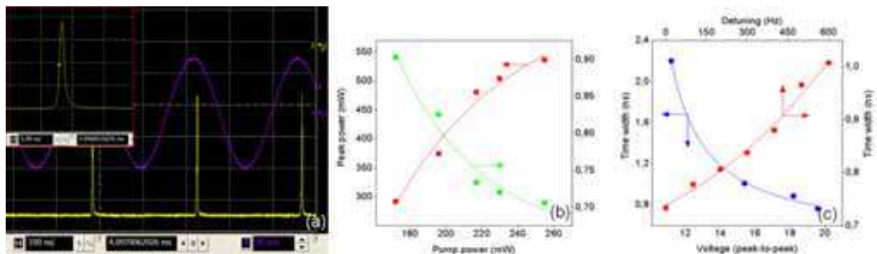
Fig. 23. (a) Oscilloscope traces of the sinusoidal electrical signal applied to the piezoelectric at 4.1 MHz repetition rate and 16 V (upper trace), and the train of optical pulses generated (lower trace); a pump power of 230 mW was used. The inset shows the detail of a single pulse of the optical train, with a FWHM of 720 ps and a peak power of 500 mW. (b) Peak power and pulse width (FWHM) of the optical pulses as a function of the pump power (solid and dotted curves, respectively). (c) Pulse width of the optical pulses when the applied voltage to the piezoelectric is varied, and when the frequency of the electrical signal is varied
