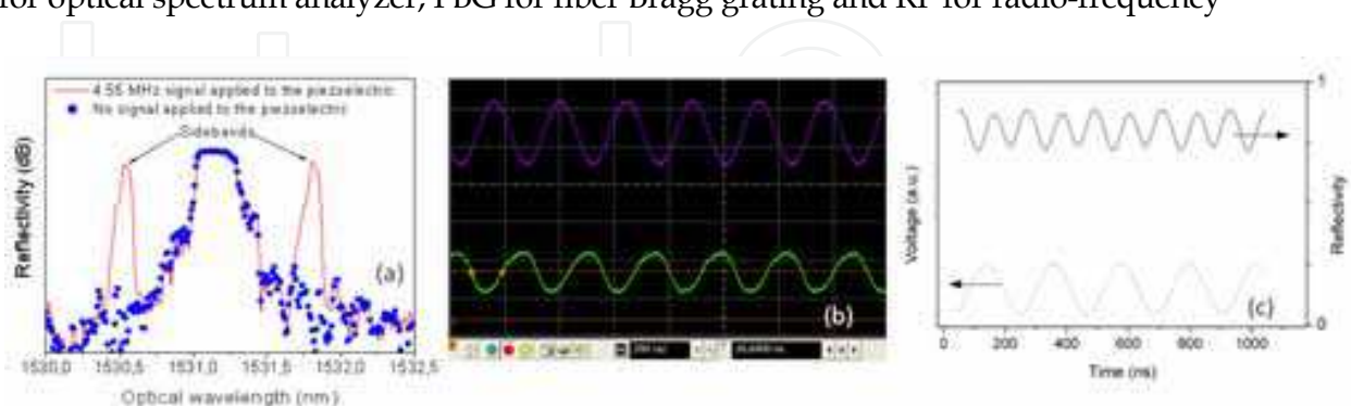
Fig. 17. (a) Reflectivity of the fiber Bragg grating with and without electrical signal applied to the piezoelectric (4.55 MHz and 16 V peak-to-peak). (b) Optical signal reflected by the short-wavelength sideband when travelling acoustic waves are used (lower trace) and RF voltage applied to the piezoelectric (4.11 MHz and 16 V, upper trace). (c) Same as in (b), but for standing acoustic waves (4.55 MHz and 16 V, dotted curve)
