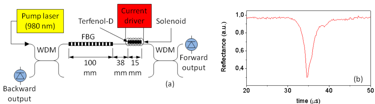
Fig. 28. (a) Q -switched distributed feedback-fiber laser setup. (b) Reflection at the Bragg wavelength when an acoustic pulse travels along the FBG
