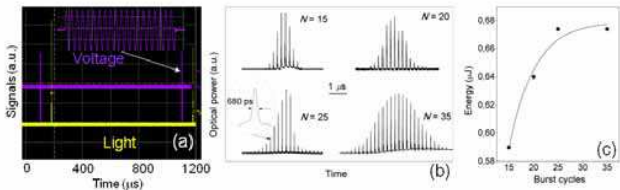
Fig. 24. (a) Voltage signal applied to the piezoelectric and Q -switched mode-locked train of pulses generated for a 1 kHz Q -switching repetition rate; the inset shows a detail of the burst signal. (b) Single Q -switched mode-locked pulses enveloping a train of modelocked pulses for different burst cycles; the inset shows a single-shot capture of a single modelocked pulse with a FWHM of 680 ps. (c) Energy of the Q -switched mode-locked pulses as a function of the cycles contained in the burst for a fixed Q -switching frequency of 500 Hz and a pump power of 270 mW
