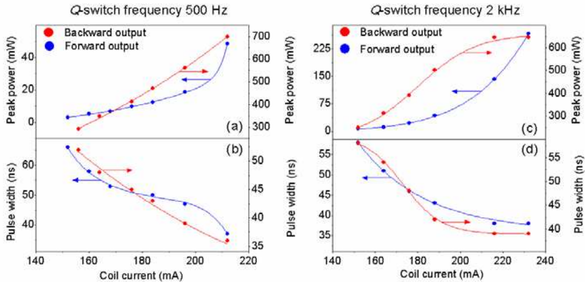
Fig. 30. Peak power and pulse width for backward and forward outputs as a function of the coil current for two different Q -switched repetition rates: 500 Hz (a, b) and 2 kHz (c, d), respectively, and 55mW of pump power
