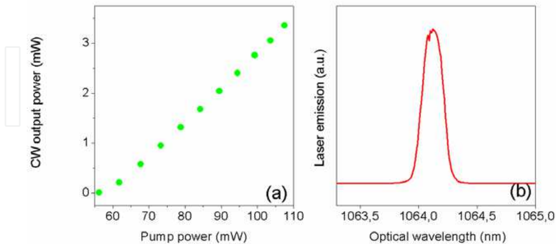
Fig. 3. (a) Output optical power in CW emission as a function of the pump power. (b) Emission spectrum
