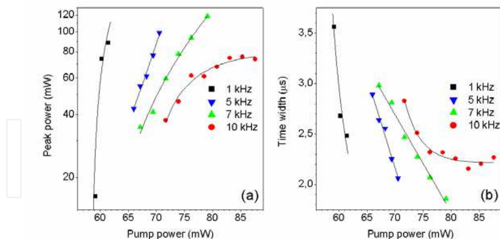
Fig. 5. Peak power and time width in Q -switched operation as a function of the pump power, (a) and (b), respectively, for several repetition rates
