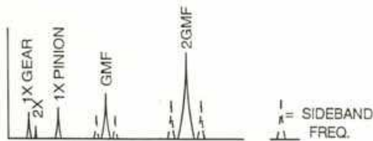
Fig. 5. Spectrum indicating misalignment of gear
