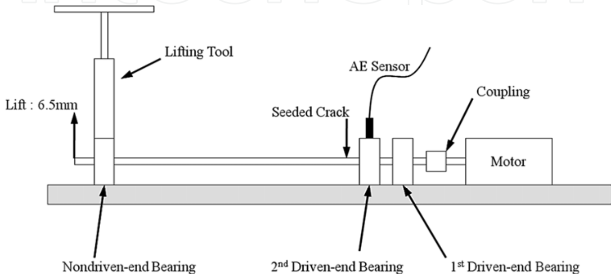
Fig. 12. Experiment system
