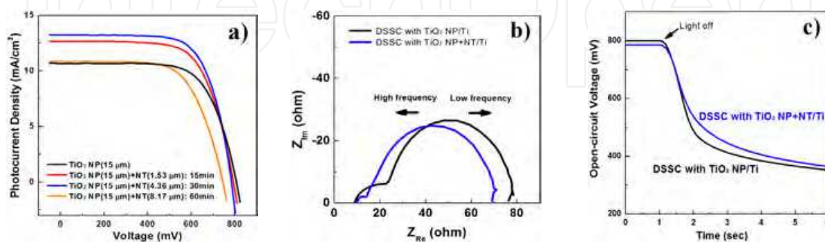
Fig. 11. (a) J - V characteristics of the DSSC with TiO 2 NP/Ti and TiO 2 NP + NT/Ti. (b) Electrochemical impedance spectra in frequencies ranging from 10 -1 to 10 6 Hz. (c) Open-circuit voltage decay measurement. © The Royal Society of Chemistry [19] .
