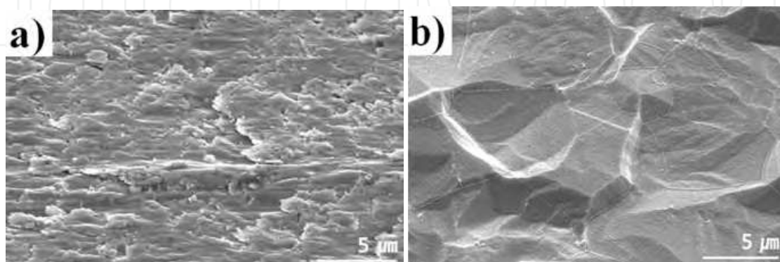
Fig. 4. SEM images of the Ti surface before thermal annealing: (a) non-treated, (b) HF- \text{HNO}_3 treated. © WILEY-VCH Verlag GmbH & Co. KGaA, Weinheim [18] .
