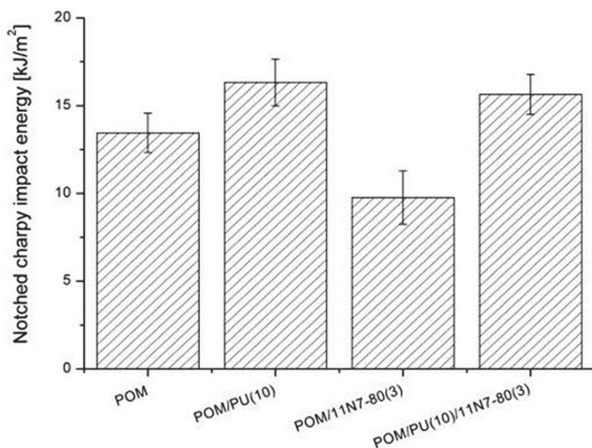
Fig. 20. the impact energy for the composites produced by water-assisted extrusion melt compounding model (Siengchin et al., 2008).
