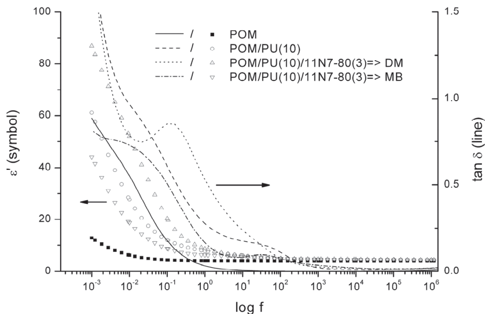
Fig. 12. Dielectric permittivity ( \epsilon' ) and dissipation factor ( \tan \delta ) as a function of frequency ( f ) for the composites produced by masterbatch (MB) and direct melt compounding (DM) (Siengchin et al., 2008).
