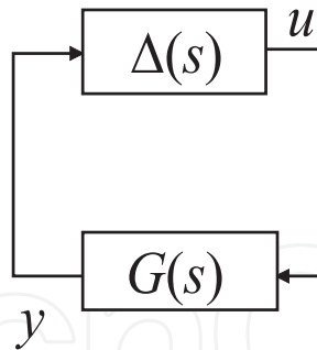
Fig. 1. Interconnection of a plant and time delay
