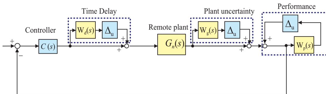
Fig. 16. Block diagram of the system with the conventional controller
