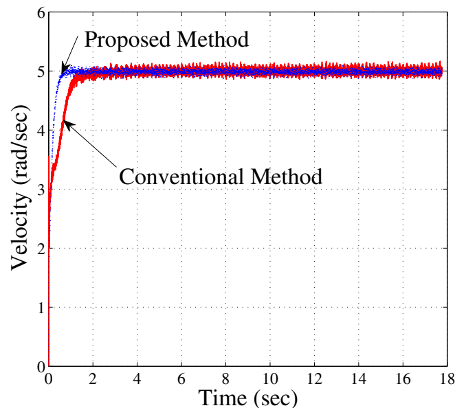
Fig. 17. Experimental results (Step response of velocity control)
