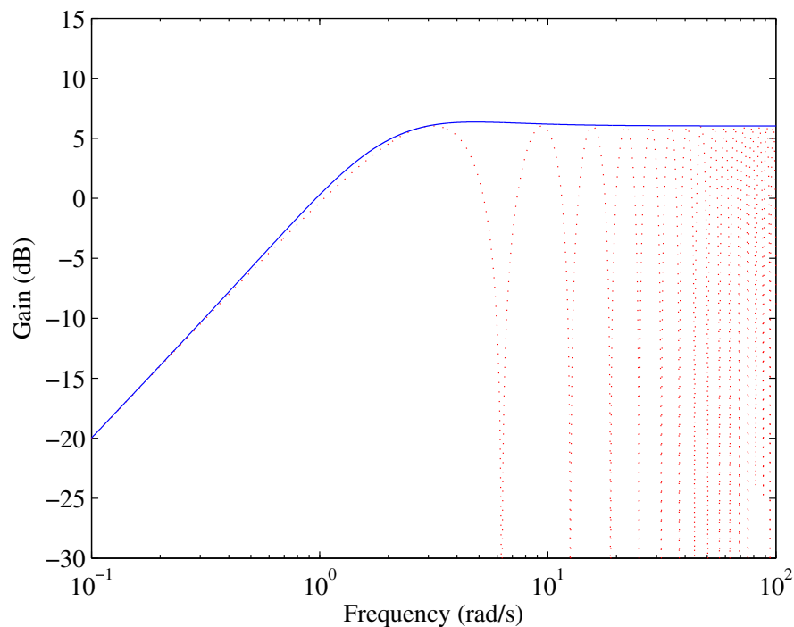
Fig. 4. Bode plots of W_d(s) (blue line) and e^{-Ts} - 1 (red dotted line)
