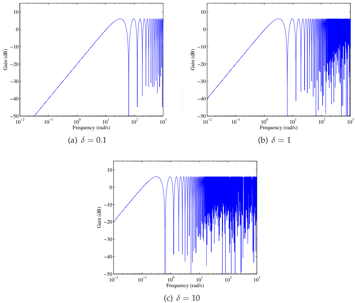
Fig. 3. Bode plot of e^{-\delta s} - 1
