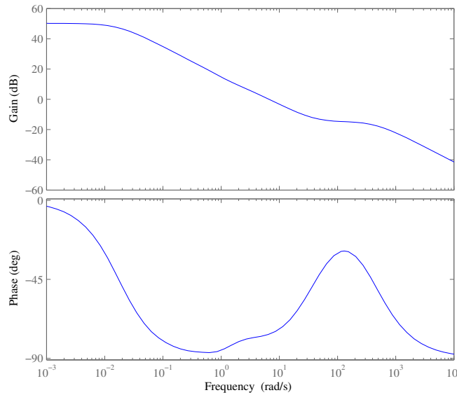
Fig. 15. Bode plot of the controller C(s)
