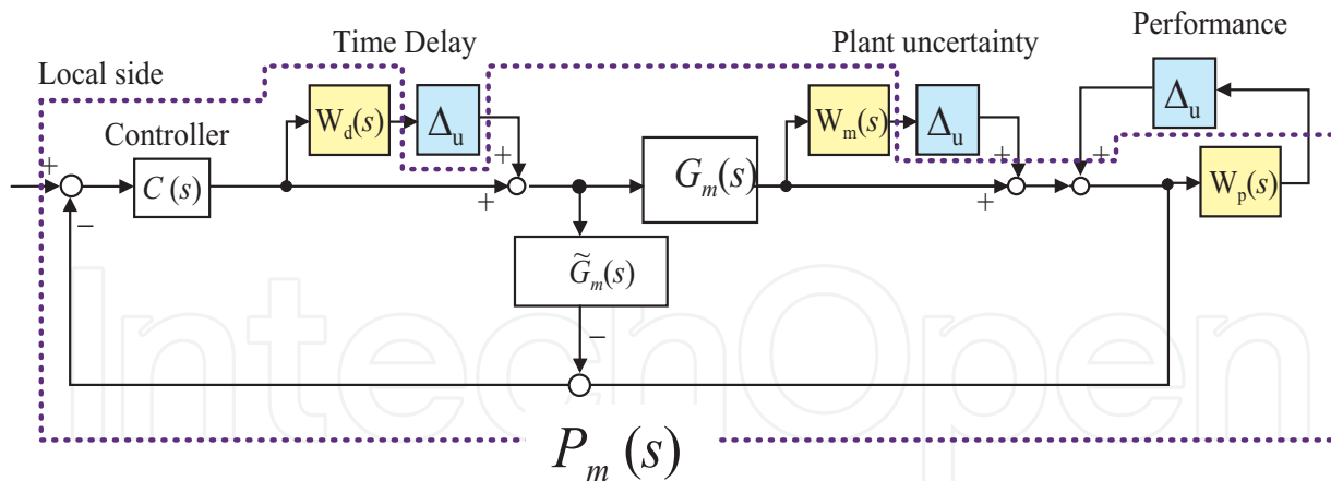
Fig. 10. Augmented plant P_m
