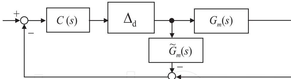
Fig. 8. Model based control structure
