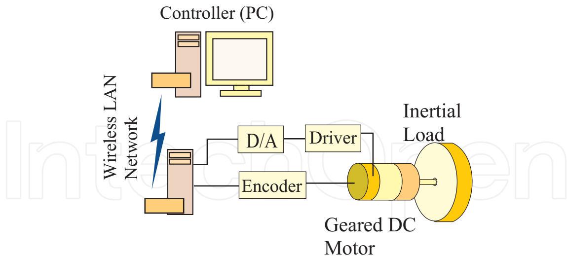
Fig. 12. Experimental setup and system configuration
