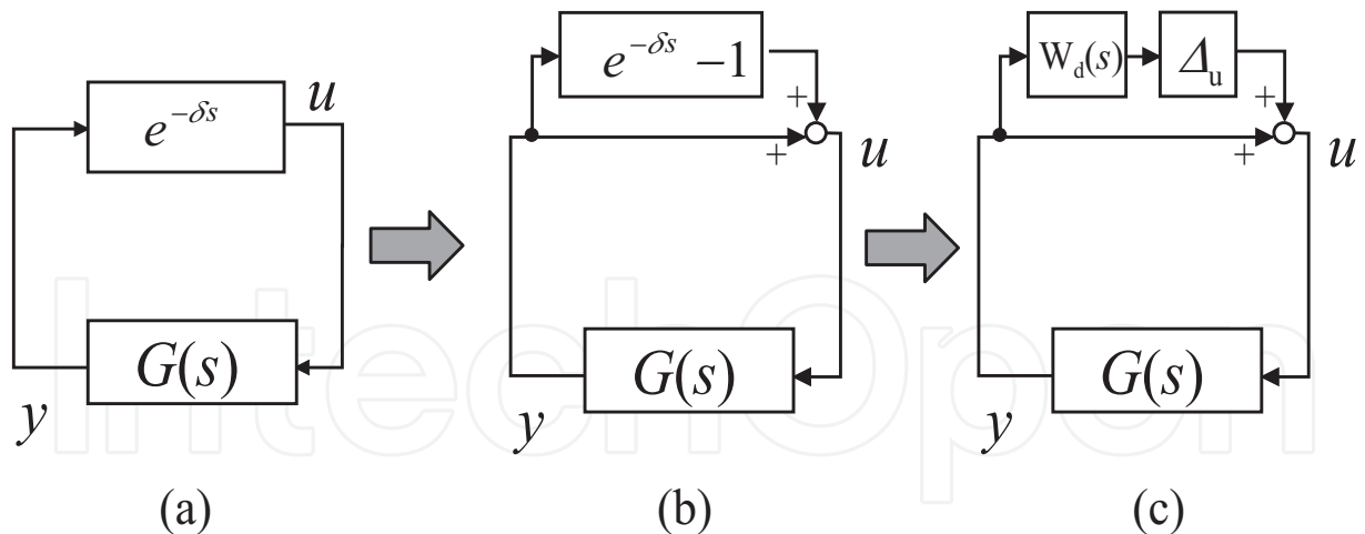
Fig. 2. Robust control based method
