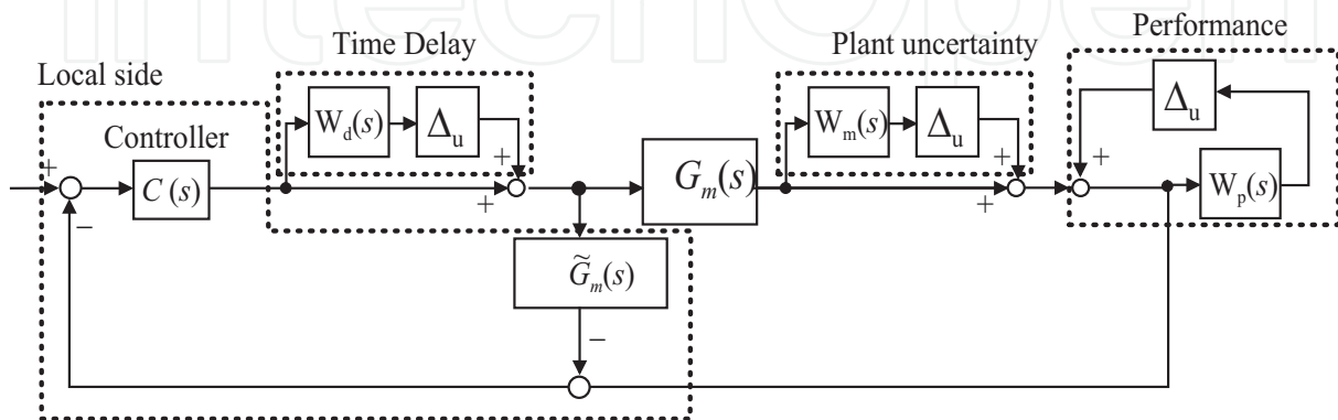
Fig. 9. Overall structure with perturbations
