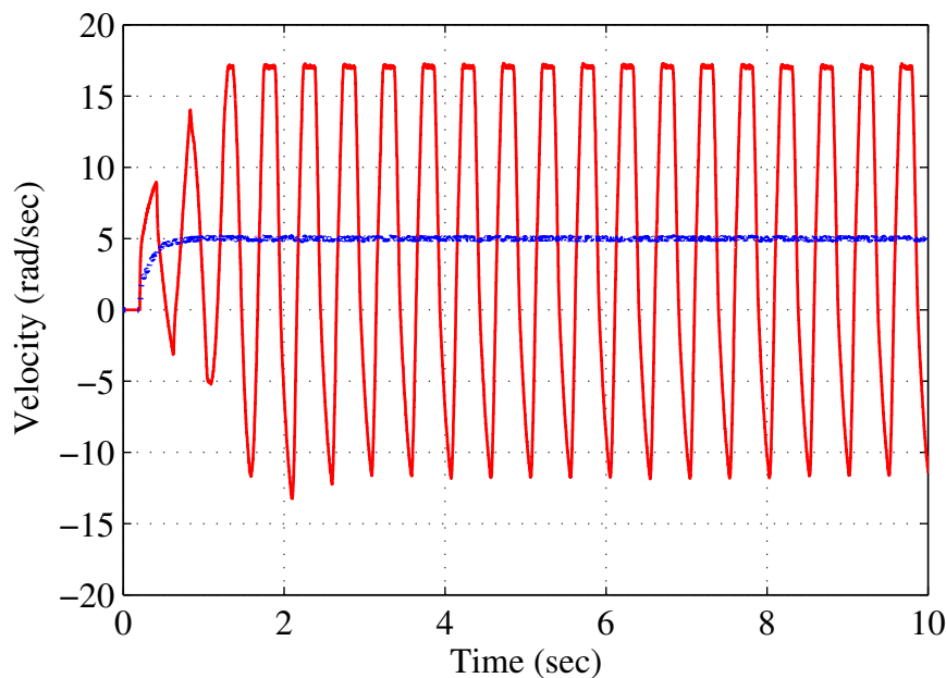
Fig. 18. Experimental results (with intentionally added delay)
