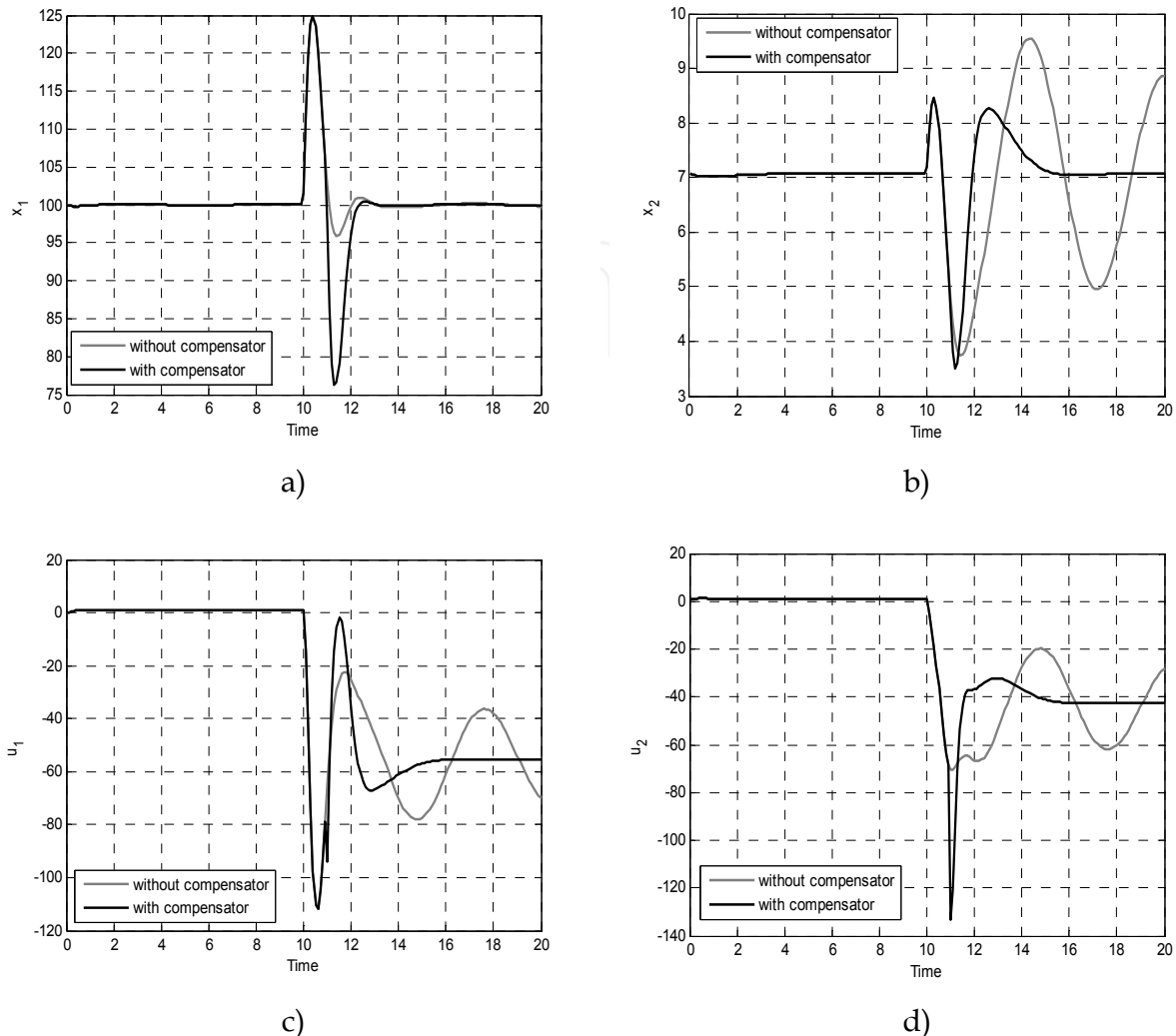
Fig. 8. Output disturbance rejection using robust nonlinear controller and feed-forward compensator considering time delay measurements of the disturbance d a) x_1 b) x_2 c) u_1 d) u_2
