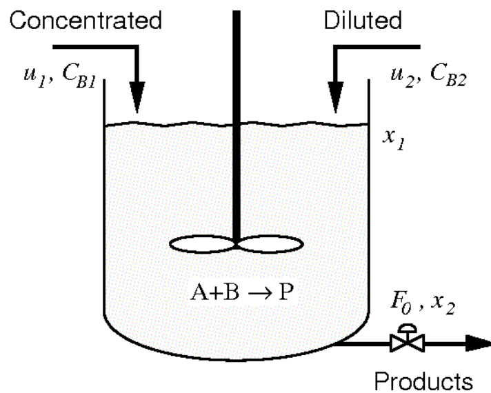
Fig. 5. Continuous stirred tank reactor (De Oliveira, 1994)
