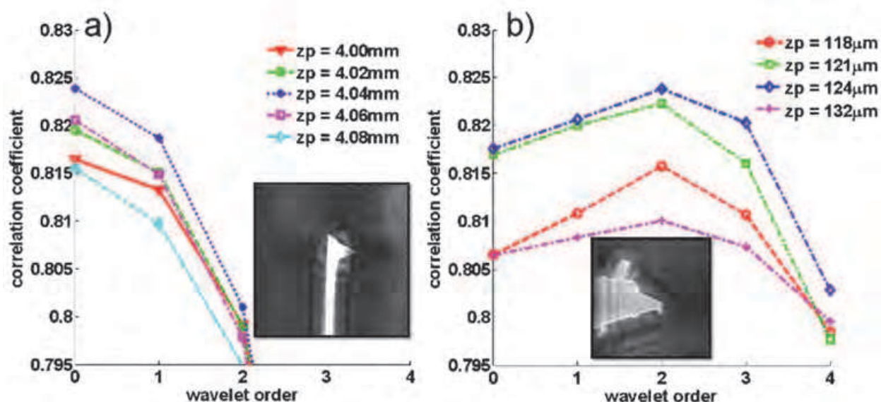
Fig. 6. Correlation values for different object-hologram distances z_p as a function of the wavelet scale X , a) recording with NA=0.038 , pixel size 270 nm, b) recording with NA=0.172 , pixel size 41 nm.
